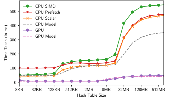
Figure 13: Join Performance.
