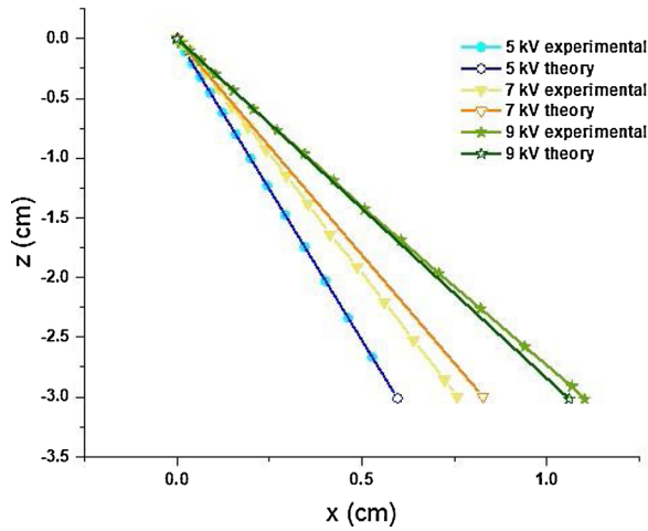
Fig. 11. Droplet trajectories in the case of charging by ionized air as in Fig. 1b. Experimental data are shown by symbols, the trajectories predicted by Eq. (6)-by straight lines with open symbols corresponding to the listed applied voltages.
