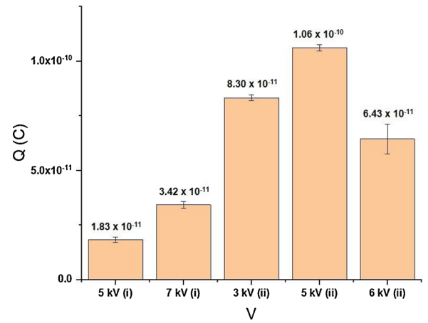
Fig. 8. The average charge of glycerol droplets found using Eq. (7) and the experimentally measured droplet landing location. Charging by ionized air is denoted as (i), whereas direct charging by wire electrode as (ii).
