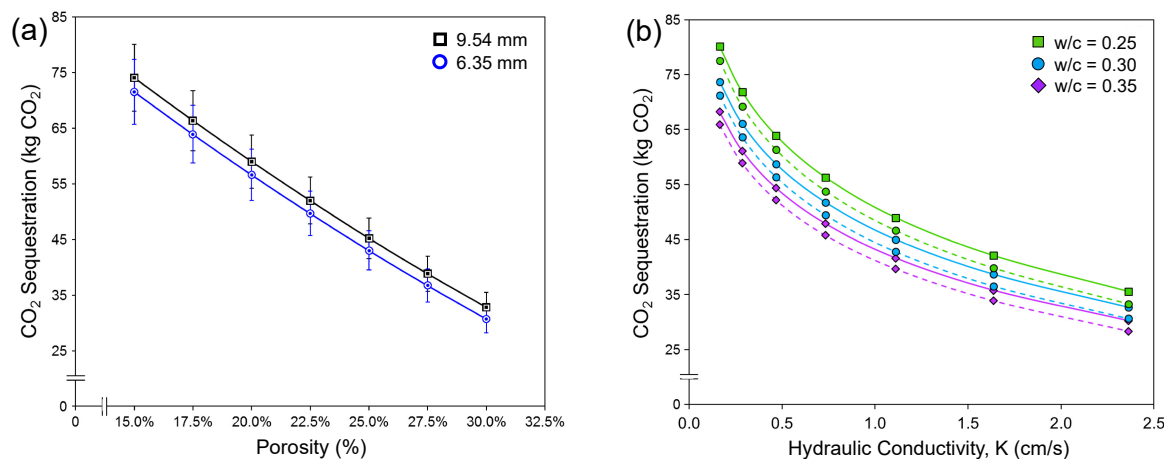
Figure 5. (a) Effect of design porosity on average CO 2 sequestration of 1 m 3 of pervious concrete. Means and error bars represent \pm one standard deviation of CO 2 sequestration potential from fixed-porosity mixtures designed using water-to-cement ( w/c ) ratios of 0.25, 0.30, and 0.35. Aggregate size is differentiated by color. (b) Effect of design hydraulic conductivity on average CO 2 sequestration potential of a 1 m 3 of pervious concrete, with varying w/c ratios and both 9.35 mm (—) and 6.35 mm (---) aggregate.
