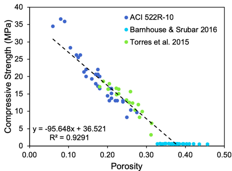
Figure 1. Relationship between compressive strength and porosity [4,10,38].
