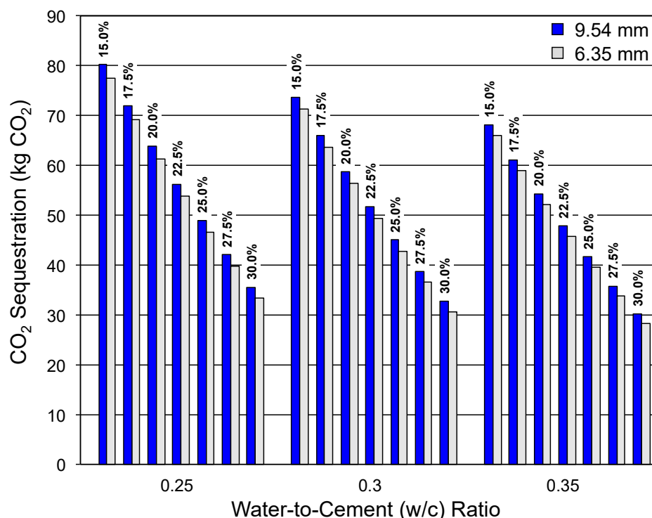
Figure 3. CO 2 sequestration potential for 1 m 3 of pervious concrete. Design porosity of each mixture is indicated above its respective column. Aggregate size is differentiated by color.
