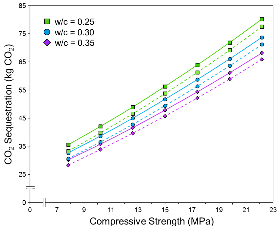
Figure 4. Effect of compressive strength on the CO 2 sequestration potential of 1 m 3 of pervious concrete with varying water-to-cement (w/c) ratios and both 9.35 mm (—) and 6.35 mm (---) aggregate.
