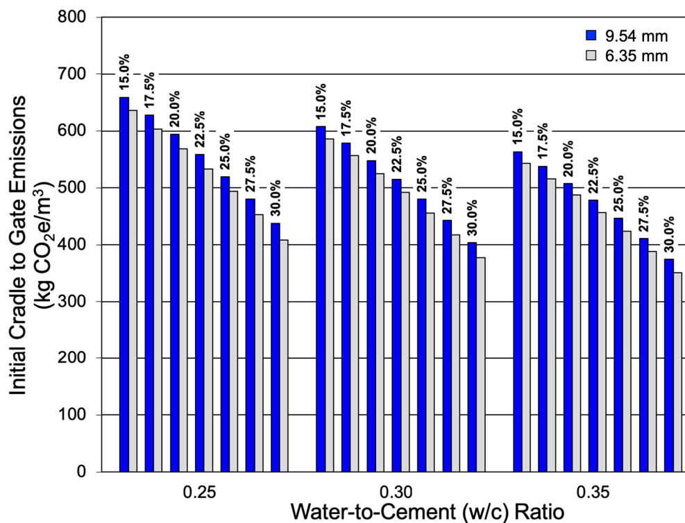
Figure 2. Initial cradle-to-gate CO 2 e emissions of pervious concrete mixtures designed according to the NRMCA design methodology [35,36]. Design porosity of each mixture is indicated above its respective column. Aggregate size is differentiated by color.
