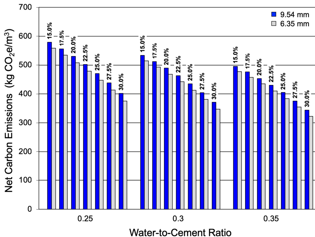
Figure 6. Net CO 2 e emissions of 1 m 3 of pervious concrete. Design porosity of each mixture is indicated above its respective column. Aggregate size is differentiated by color.
