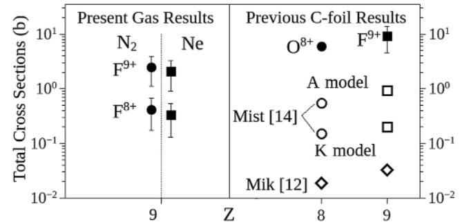
FIG. 6. Present results for N 2 and Ne targets (left-hand panel). Previous results for fully stripped projectiles on thin-foil C targets (right-hand panel). The cross sections obtained for the C targets are uncertain due to multiple collisions (see text). The A and K models of the theory are from Ref. [14].
