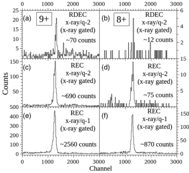
FIG. 3. Spectra for 2.11 MeV/u F^{9+} (left) and F^{8+} (right) + N_2 . (a),(b) x-ray/q-2 events from Fig. 2(b) sorted on x rays from the RDEC energy range [Fig. 2(a)], (c),(d) x-ray/q-2 events from Fig. 2(b), and (e),(f) x-ray/q-1 events from Fig. 2(c) sorted on x rays from the REC energy range [Fig. 2(a)].
