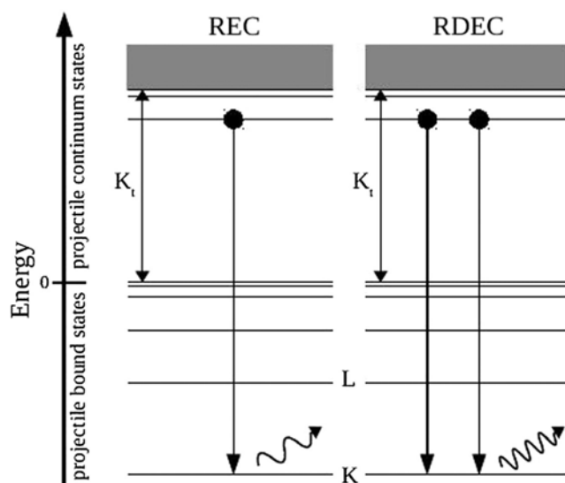
FIG. 1. Energy schematic for the radiative capture of one (REC) or two (RDEC) electrons from a target bound state. K_t is the kinetic energy of the captured electron(s) as seen from the projectile reference frame. The captured electrons can go to any available projectile shell.
