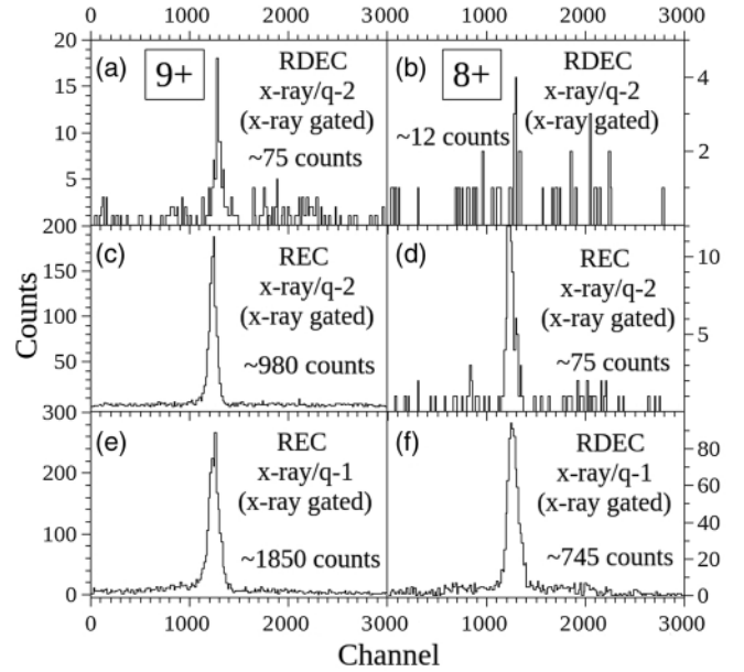
FIG. 4. Spectra for 2.11 MeV/u F^{9+} (left) and F^{8+} (right) + Ne. (a),(b) x-ray/q-2 events from spectra similar to Fig. 2(b) sorted on x rays from the RDEC energy range [spectrum like Fig. 2(a)], (c), (d) x-ray/q-2 events from spectra like Fig. 2(b), and (e),(f) x-ray/q-1 events from spectra like Fig. 2(c) sorted on x rays from the REC energy range [spectrum like Fig. 2(a)].
