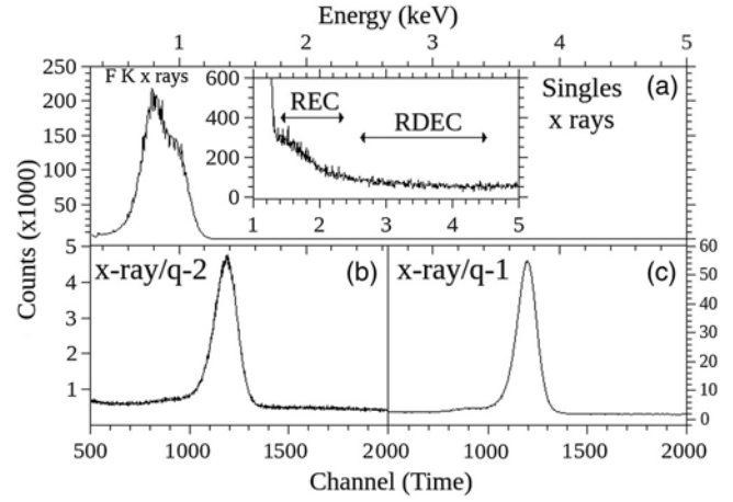
FIG. 2. Sums of collected (a) x-ray singles events, (b) x-ray/doubly charge-changed (q-2), and (c) x-ray/singly charge-changed (q-1) coincidence events for 2.11 MeV/u F^{9+} + N_2 .
