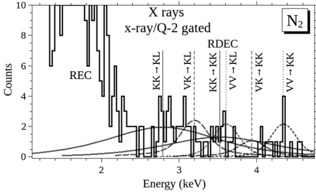
FIG. 5. X-ray spectrum obtained from events sorted on the x-ray/q-2 coincidence spectrum [Fig. 2(b)] for 2.11 MeV/u F 9+ incident on N 2 . The smooth curves under the RDEC region show the calculated Compton profiles of the transitions arbitrarily normalized to the data. The following scheme is used based on the initial state of the transition: VV is indicated by the short dashed lines, VK by the long dashed lines, and KK by the solid lines.
