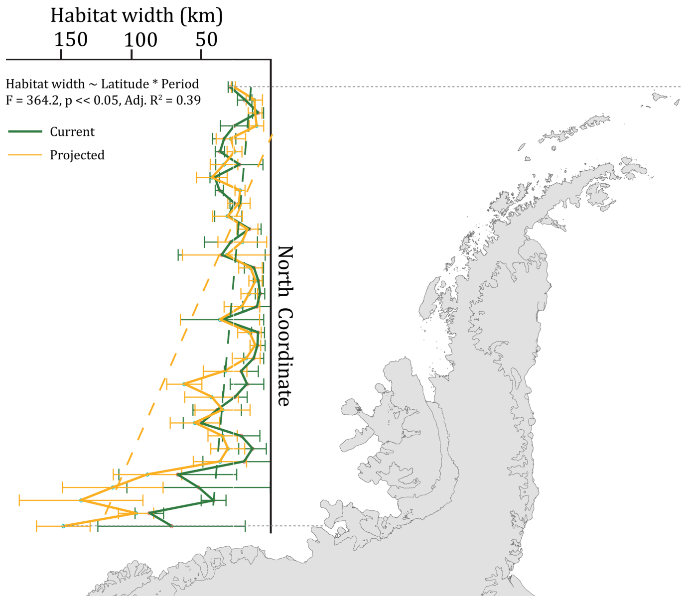
Extended Data Fig. 2 | Projected expansion in habitat. Projected future offshore expansion of the habitat of crabeater seals along the western Antarctic Peninsula (Linear regression model: Habitat width ~ Latitude * Period ). Habitat width was defined as the mean distance between the coast and the 50% habitat importance contour for 50 km bins in the North coordinate. Error bars indicate the standard deviation of the habitat width for the bins. Colour dashed lines indicate the fitted linear regressions. Green indicates current habitat width. Yellow is projected habitat width under projected environmental changes.
