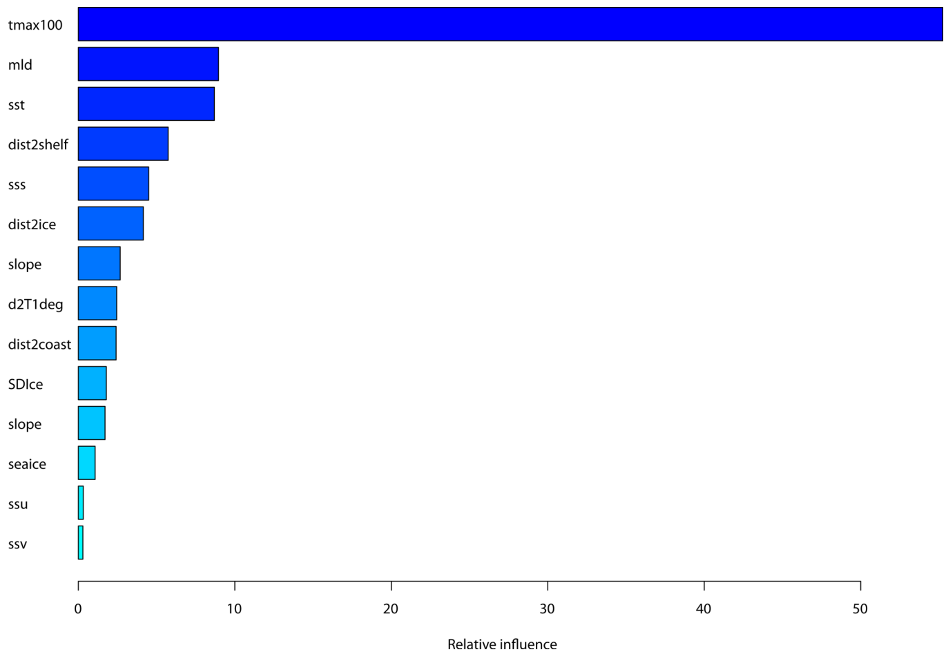
Extended Data Fig. 6 | Boosted Regression Trees - Variable Influence. Boosted Regression Tree (BRT) Analysis. Relative influence of environmental variables used in the BRT models to predict foraging habitat of crabeater seals. The relative influence indicates the proportion of variation in the data explained by each variable with respect to the rest of the variables.
