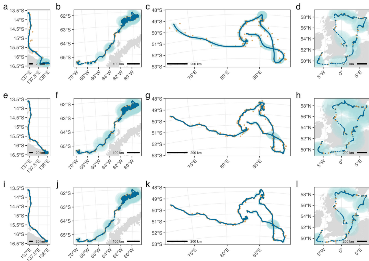
Fig. 2 State-space model fits to the three Argos satellite data types obtained from a hawksbill turtle (HBTU; a,e,i), a leopard seal (LESE; b,f,j), a southern elephant seal (SESE; c,g,k), and a northern gannet (NOGA; d,h,l). State-space model-predicted locations (dark blue points) smooth through the Argos data types (gold points) - Least-Squares (a,b,c,d), Kalman filter (e,f,g,h) and Kalman smoother (i,j,k,l) - at regularly specified 2-h intervals. The 95% confidence intervals on the predicted locations (light blue shading) are also displayed. Spatial scale in km is indicated at lower left or right of each panel
