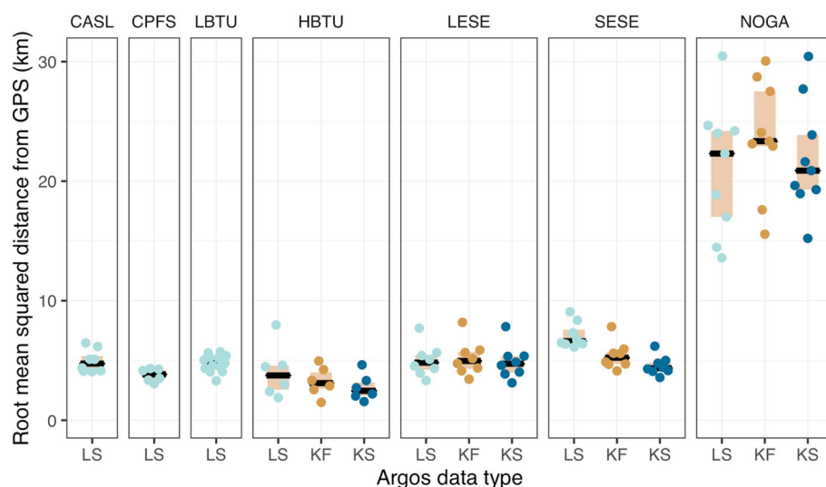
Fig. 3 Accuracy of state-space model-estimated locations across the three Argos location data types and by species. Accuracy is assessed using root mean squared distance (RMSD in km) from interpolated GPS locations. Individual RMSD values are filled circles, coloured by Argos data type, beige boxes are inner quartile ranges, and black bars are medians. Species codes: CASL - California sea lion; CPFS - Cape fur seal; LBTU - leatherback sea turtle; HBTU - hawksbill sea turtle; LESE - leopard seal; SESE - southern elephant seal; NOGA - northern gannet
