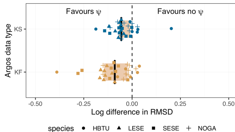
Fig. 4 Accuracy of estimated locations from models fit with and without a \psi parameter to re-scale Argos error ellipse sizes. The log difference in root mean squared distance ( \log \Delta RMSD) from interpolated GPS locations was calculated for the two models fit to each individual animal. Negative values indicate the model with a \psi parameter is more accurate, whereas positive values indicated the model without a \psi parameter is more accurate. Results are pooled across species with individual log differences in RMSD displayed as species-specific shapes (gold, blue). The inner quartile ranges are beige boxes and medians are black bars
