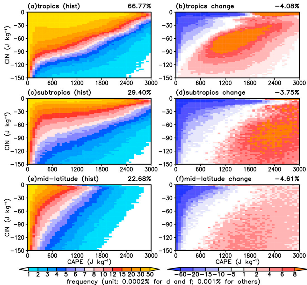
FIG. 5. (left) 1980–99 mean occurrence frequency (in % of time) of given CAPE ( x axis) and CIN ( y axis) values over land in different regions for summer (JJA for the Northern Hemisphere and DJF for the Southern Hemisphere), and (right) its change (in % of time) from 1980–99 to 2081–2100 calculated using 6-hourly data from CCSM4 simulations under the historical and RCP8.5 scenario. Note that the colored values need to be multiplied by 0.001 for all panels except for (d) and (f), which should be multiplied by 0.0002. The regions include the (a),(b) tropics ( 20^{\circ}\text{S} – 20^{\circ}\text{N} ), (c),(d) subtropics ( 20^{\circ} – 40^{\circ}\text{S/N} ), and (e),(f) midlatitudes ( 40^{\circ} – 60^{\circ}\text{S/N} ). A fixed bin number of 50 was used for both CAPE (with a bin size of 60 \text{ J kg}^{-1} ) and CIN (with a bin size of 3 \text{ J kg}^{-1} ). The total frequency or its change integrated (after the scaling) over all bins (i.e., under a limited range of CAPE and CIN, 0 < \text{CAPE} \leq 3000 \text{ J kg}^{-1} , -150 \text{ J kg}^{-1} \leq \text{CIN} < 0 ) is shown on the top-right corner of each panel. Each pair of 6-hourly CAPE and CIN values at each grid box were taken as one occurrence and all the occurrences within the time period and geographic domain were combined to produce the frequency distributions without any averaging.
