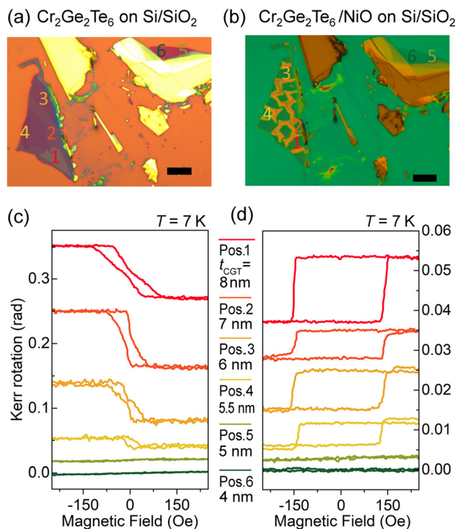
FIG. 1. (a) and (b) Optical microscopy image of \text{Cr}_2\text{Ge}_2\text{Te}_6 (CGT) flakes on a Si/SiO 2 substrate, before (a) and after (b) the deposition of NiO. After the deposition of NiO with a thickness of 20 nm, the optical contrast changes because the interference condition is modified. The scale bar is 10 \mu\text{m} . (c) Measured magneto-optical Kerr effect (MOKE) curves at the temperature of 7 K, with the magnetic field perpendicular to the substrate. The curves from different positions (labeled 1–6) are shifted vertically. The positions are marked in the images (a) and (b). The CGT-flake thickness at each position was measured by atomic force microscopy. (d) MOKE curves measured at the same positions after NiO deposition. Perpendicular anisotropy is strongly enhanced, and square shaped hysteresis curves are observed. The opposite sign of the MOKE hysteresis curves between (c) and (d) is supposedly due to the different optical constants of the sample without (c) and with (d) the NiO overlayer. 14
