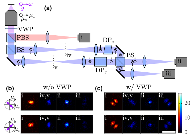
FIG. 7. (a) A single-objective interferometric imaging system that reaches the quantum limit of measurement precision. A vortex wave plate (VWP) is placed at the BFP to convert radially and azimuthally polarized light to x - (blue) and y -polarized (red) light, respectively, which is then separated by a polarizing beam splitter (PBS). Camera (i) detects an azimuthally polarized image identical to those captured by cameras (i) and (ii) in Fig. 2. The radial channel is split and recombined by a pair of 50:50 beam splitters (BS) in a Mach-Zehnder configuration; light in each arm is flipped using orthogonally oriented dove prisms (DPs). Cameras (ii) and (iii) detect images identical in shape but half as bright as those captured by cameras (iii) and (iv) in the dual-objective system in Fig. 2. [(b), (c)] Images of molecules with orientations -\mu_x = \mu_y = \mu_z and \mu_x = \mu_y = \mu_z captured at detectors (i)–(iii) and intermediate image planes (iv) and (v) both (b) without and (c) with VWPs. Images depict a total of 2000 photons detected. Scale bar: 1 \mu\text{m} . Color bar: photons per 58.5 \times 58.5 \text{ nm}^2 pixel.
