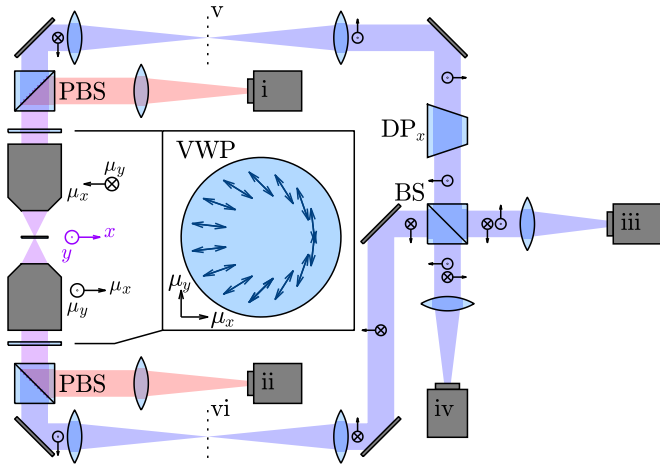
FIG. 2. Dual opposing-objective interferometric imaging (dualObj) for achieving QCRB-limited precision. Two vortex (half-) wave plates (VWP) are placed at the BFPs to convert radially polarized to x -polarized light (blue) and azimuthally polarized to y -polarized light (red). Blue arrows depict the fast axis direction of the VWP. One of the radially polarized channels is flipped using an x -oriented Dove prism (DP) and then propagates to the beam splitter (BS).
