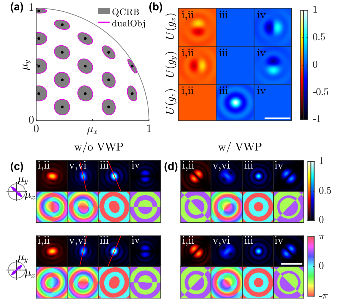
FIG. 3. Estimation precision and optical fields produced by the dual objective interferometric imaging system. (a) CRB covariance ellipses for measuring [\mu_x, \mu_y] using 25 detected photons and interferometric detection (magenta) compared to the quantum bound. To compute the covariance for N photons detected, scale the dimensions of the ellipses by 5/\sqrt{N} . (b) Basis electric fields U(g_x) , U(g_y) , and U(g_z) at detectors (i)–(iv) in Fig. 2. [(c), (d)] Normalized amplitude and phase of the optical fields of molecules with orientations -\mu_x = \mu_y = \mu_z and \mu_x = \mu_y = \mu_z captured at detectors (i)–(iv) and intermediate image planes (v) and (vi) in Fig. 2 (c) without and (d) with VWPs. Scale bar: 1 \mu\text{m} . Color bars: normalized amplitude and phase in rad.
