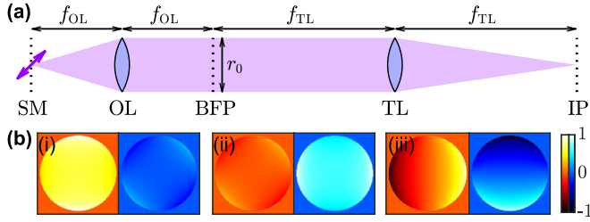
FIG. 6. Overview of a simplified two-lens imaging system. (a) An objective lens (OL) captures light emitted by a single-molecule (SM) emitter positioned at its focal plane. A tube lens (TL) is used to focus light to the image plane (IP). (b) Basis electric fields (i) g_x , (ii) g_y , and (iii) g_z at the back focal plane (BFP) of the imaging system normalized to the maximum amplitude of g_x . Red, x -polarized field; blue, y -polarized field.
