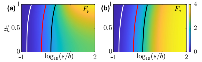
FIG. 10. Quantum FI of estimating first-order orientational moments of fixed dipole emitters as a function of signal-to-background ratio (SBR). (a) QFI of estimating polar orientation. (b) QFI of estimating azimuthal orientation. Black, red, and white lines represent a QFI reduction of 50%, 75%, and 96%, i.e., a best possible standard deviation in the presence of background equal to \sqrt{2} , two, and five times that without background, respectively.
