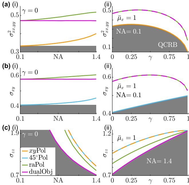
FIG. 4. Classical CRB of several techniques (Appendix E) compared to the quantum CRB of estimating second-order orientational moments of dipole emitters. (a) CRB SGV of estimating M_{xx} and M_{yy} for molecules wobbling around the \mu_x axis, [(b), (c)] best-possible precision \sqrt{\text{CRB}} of estimating (b) M_{xy} for molecules wobbling around the \mu_x axis and (c) M_{zz} for molecules wobbling around the \mu_z axis as functions of (i) numerical aperture NA (for \gamma = 0 ) and (ii) rotational constraint \gamma [NA = 0.1 in (a) and (b) and NA = 1.4 in (c)]. The gray regions are bounded from above by (a) QCRB or [(b), (c)] \sqrt{\text{QCRB}} [Eq. (18)]. Orange, standard PSF with x - and y -polarized detection (xyPol); cyan, standard PSF with linearly polarized detection at \pm 45^\circ in the xy plane (45Pol); green, standard PSF with radially and azimuthally polarized detection (raPol); and magenta, dual-objective interferometric detection with VWP (dualObj). All curves assume one photon is detected from the dipole emitter. For N photons detected, scale the vertical axis values by (a) 1/N and [(b), (c)] 1/\sqrt{N} . The estimation precision of 45Pol in panel (a) and xyPol in panel (b) are orders of magnitude larger than those of the other techniques and are not shown.
