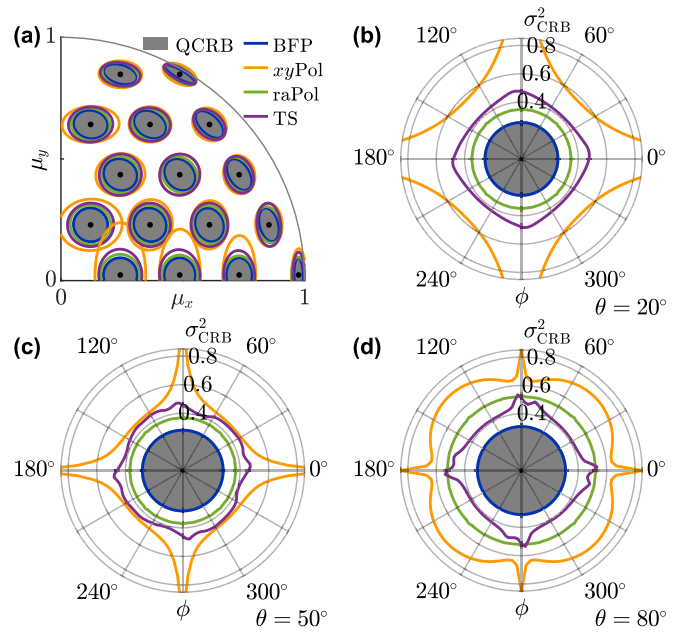
FIG. 1. Classical CRB of several techniques (Appendix B) compared to the quantum CRB of estimating first-order orientational moments of fixed dipole emitters. (a) CRB covariance ellipses for measuring [\mu_x, \mu_y] using 25 detected photons. To compute the covariance for N photons detected, scale the dimensions of the ellipses by 5/\sqrt{N} . [(b)–(d)] CRB standardized generalized variance (SGV in steradians) \sigma_{\text{CRB}}^2 = [\mu_z^2 \det(\mathcal{J})]^{-1/2} of estimating [\mu_x, \mu_y] , normalized to quantify orientation precision as a solid angle on the surface of a unit sphere. SGV is computed for a dipole with orientation (b) \theta = 20^\circ , (c) \theta = 50^\circ , and (d) \theta = 80^\circ and one photon detected. For N photons detected, SGV may be computed by scaling the radial axis by 1/N . The gray regions are bounded from above by QCRB [Eqs. (12) and (14)]. Blue, direct BFP imaging (BFP); orange, standard PSF with x - and y -polarization separation ( xy\text{Pol} ); green, standard PSF with radial- and azimuthal-polarization separation (raPol); and purple, tri-spot PSF with x - and y -polarized detection (TS).
