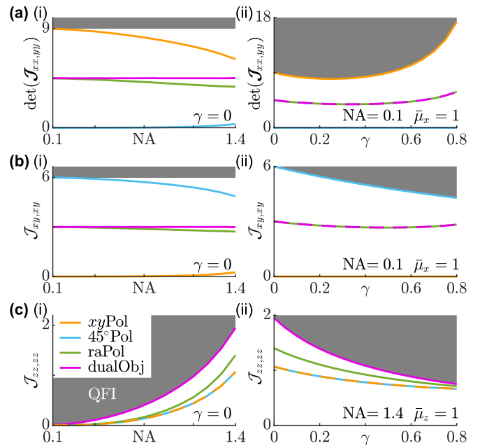
FIG. 9. Classical FI of several techniques (Appendix E) vs quantum FI of estimating second-order orientational moments of dipole emitters. (a) Inverse of generalized variance for estimating M_{xx} and M_{yy} , classical FIs for estimating (b) M_{xy} for molecules wobbling around the \mu_x axis, and (c) M_{zz} for molecules wobbling around the \mu_z axis as functions of (i) numerical aperture NA (for \gamma = 0 ) and (ii) rotational constraint \gamma [for (a),(b) NA = 0.1 and (c) NA = 1.4]. The gray regions are bounded from below by the QFI [Eq. (18)]. Orange, standard PSF with x - and y -polarized detection (xyPol); cyan, standard PSF with linearly polarized detection at \pm 45^\circ in the xy plane (45Pol); green, standard PSF with radially and azimuthally polarized detection (raPol); and magenta, dual-objective interferometric detection with VWP (dualObj). All curves assume one photon is detected from the dipole emitter.
