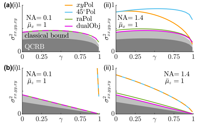
FIG. 5. CRB standardized generalized variance (SGV in steradians) of estimating in-plane moments M_{xx} , M_{yy} , and M_{xy} simultaneously for molecules wobbling around the (a) \mu_x axis and (b) \mu_z axis using (i) NA = 0.1 and (ii) NA = 1.4 objective lenses. The dark gray regions are bounded from above by the quantum bound [Eq. (18)]; light gray regions are bounded from above by the classical bound [Eq. (19)]. Orange, standard PSF with x - and y -polarized detection (xyPol); cyan, standard PSF with linearly polarized detection at \pm 45^\circ in the xy plane (45Pol); green, standard PSF with radially and azimuthally polarized detection (raPol); and magenta, dual-objective interferometric detection with VWP (dualObj). All curves assume one photon is detected from the dipole emitter. For N photons detected, scale the vertical axis values by 1/N . The estimation precision of 45Pol and xyPol in (i) are orders of magnitude larger than those of the other techniques and are not shown.
