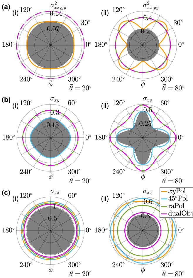
FIG. 8. Classical CRB of several techniques (Appendix E) compared to the quantum CRB of estimating second-order orientational moments of a nearly fixed ( \gamma = 0.8 ) dipole emitter with average polar orientation (i) \bar{\theta} = 20^\circ and (ii) \bar{\theta} = 80^\circ using one detected photon. (a) CRB SGV for estimating in-plane squared moments M_{xx} and M_{yy} using a low 0.1 NA objective. (b) Best-possible precision \sqrt{\text{CRB}} of estimating the in-plane cross moment M_{xy} using a low 0.1 NA objective. (c) Best possible precision \sqrt{\text{CRB}} of estimating the out-of-plane squared moment M_{zz} using a high 1.4 NA objective. The gray regions are bounded from above by the numerically computed (a) QCRB or [(b), (c)] \sqrt{\text{QCRB}} . Orange, standard PSF with x - and y -polarized detection (xyPol); cyan, standard PSF with linearly polarized detection at \pm 45^\circ in the xy plane (45°Pol); green, standard PSF with radially and azimuthally polarized detection (raPol); and magenta, dual-objective interferometric detection with VWP (dualObj). All curves assume one photon is detected from the dipole emitter. The estimation precision of 45°Pol in panel (a) and xyPol in panel (b) are orders of magnitude larger than those of the other techniques and are not shown.
