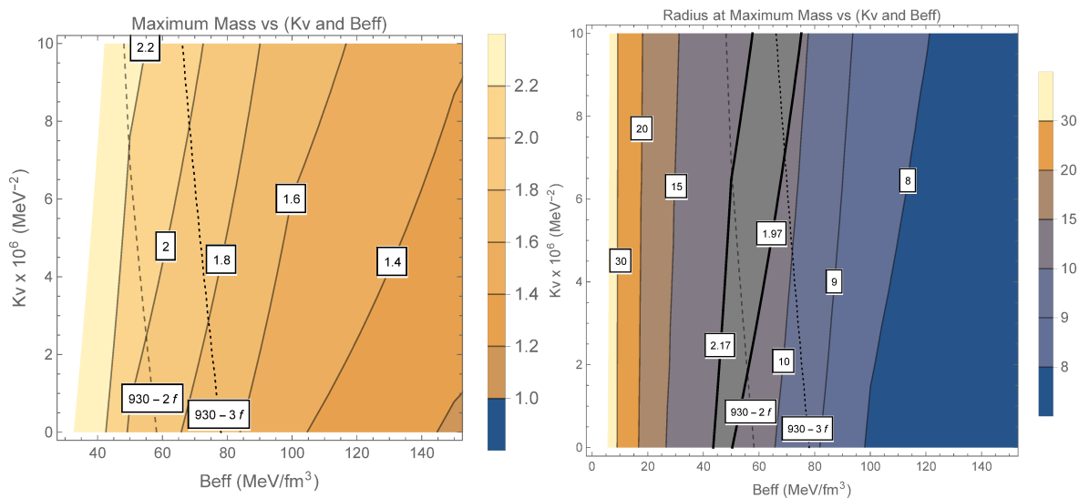
Figure 1. Contours of constant maximum mass ( left panel ) and of constant radius at maximum mass ( right panel ) in the vBag parameter model space. Also shown are the two-flavor and three-flavor lines of constant energy/baryon = 930 MeV (light dotted lines in both panels) and contours corresponding to values of maximum mass (right panel only) of two heavy neutron stars—J1614-2230 at 1.97M_{\odot} from pulsar observations [8] and the neutron star merger event GW170817 at 2.17M_{\odot} [23]. The apparent degeneracy of mass (or radius) in this parameter space is due to the fact that both parameters B_{\text{eff}} and K_v can be chosen independently to effectively soften or stiffen the equation of state beyond a desired baryon density that still admits stable strange matter.
