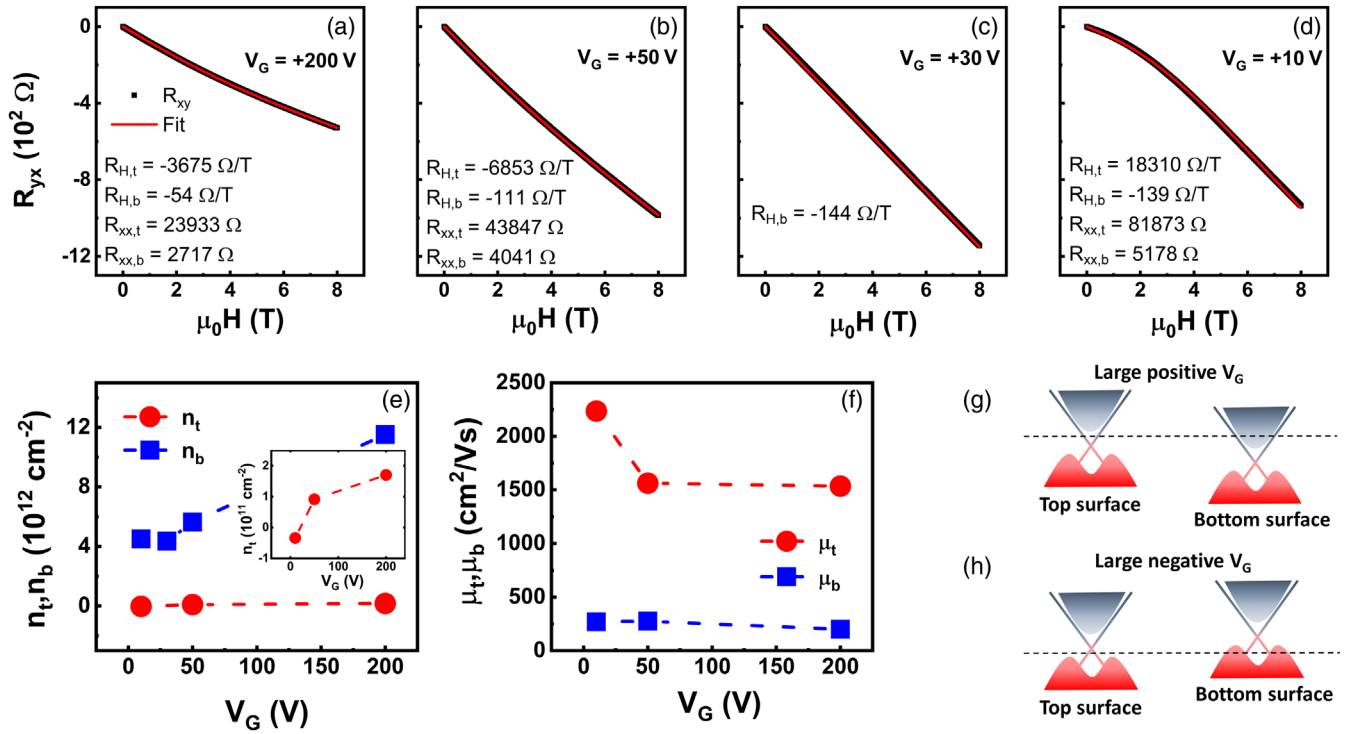
FIG. 2. (a)–(d) Two-band fittings of the Hall resistivity at V_G = +200 , +50 , +30 , and +10 V, respectively. R_{H,t} , R_{H,b} and R_{xx,t} , R_{xx,b} denote the Hall coefficients and sheet resistances for the top and bottom SSs. At V_G = +30 V, the R_{yx} curve is essentially linear, which precludes a meaningful two-band fitting. The resultant Hall coefficient from a linear fit is assigned to R_{H,b} of the bottom surface, which dominates in this transport regime. (e), (f) Carrier densities, n_t and n_b , and the corresponding mobilities \mu_t and \mu_b for the top and bottom SS at each V_G , respectively. Inset: Close-up view of n_t at each V_G . (g), (h) Schematic band structures for the top and bottom SS at large positive and negative V_G 's, respectively.
