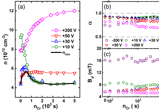
FIG. 4. (a) Electron densities at selected V_G 's with increasing Cr density for the same sample. V_G = +10 , +30 , and +50 \text{ V} are close to the surface transport regime. V_G = +200 \text{ V} serves as a reference showing the effect of electron doping by the Cr impurities. The black solid line marks the minimum electron density ( n_{\text{min}} ) identified at each n_{\text{Cr}} . (b) \alpha and (c) B_\phi from fittings of the MC data to the HLN equation at selected V_G 's as functions of Cr density.
