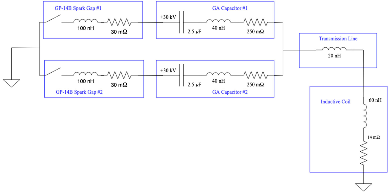
FIG. 2. MIFEDS-III circuit diagram.
