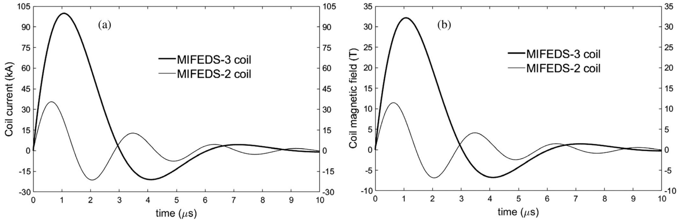
FIG. 6. Simulations of the currents and magnetic field waveforms into the 60-nH, 14-mΩ coil. Part (a) corresponds to the MIFEDS coil current and (b) shows the peak magnetic field in the coil.
