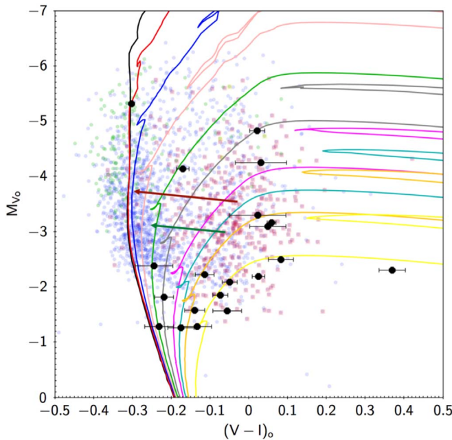
Figure 2. Example of the age determination for the HMXBs identified in field DF11 of the Chandra XVP survey. The extinction-corrected magnitude and color are defined as M_V = (m - M)_V - A_V = V - 18.96 - 0.25 , and (V - I)_0 = (V - I) - E(V - I) = (V - I) - 0.13 , respectively. The underlying points are from the spectroscopic census of OB stars in the SMC (blue B stars; green O stars, red Be stars, orange Oe stars) by Bonanos et al. (2010), overlaid with the PARSEC isochrones (black 4.5 Myr; red 6.3 Myr; blue 10.0 Myr; pink 15.8 Myr; green 25.1 Myr; gray 39.8 Myr; magenta 63.1 Myr; cyan 79.4 Myr; orange 100.0 Myr; yellow 158.5 Myr). The two vectors, maroon and dark green, show the shift of the Be stars due to their intrinsic reddening with respect to the B stars in the [B0,B2) and [B2,B4) spectral-type bins, respectively (the start and end points of the arrows are centered at the median M_V and (V - I)_0 values of each population).
