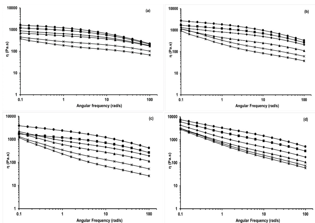
Figure 2. Complex viscosity ( \eta ) as a function of angular frequency (rad/s) at different temperatures (150–200 °C) for (a) polyacrylonitrile (PAN); (b) PAN-10%wt BL; (c) PAN-20%wt BL; and (d) PAN-30%wt BL; ●—150 °C; ■—160 °C; ◆—170 °C; ▲—180 °C; ×—190 °C; *—200 °C.
