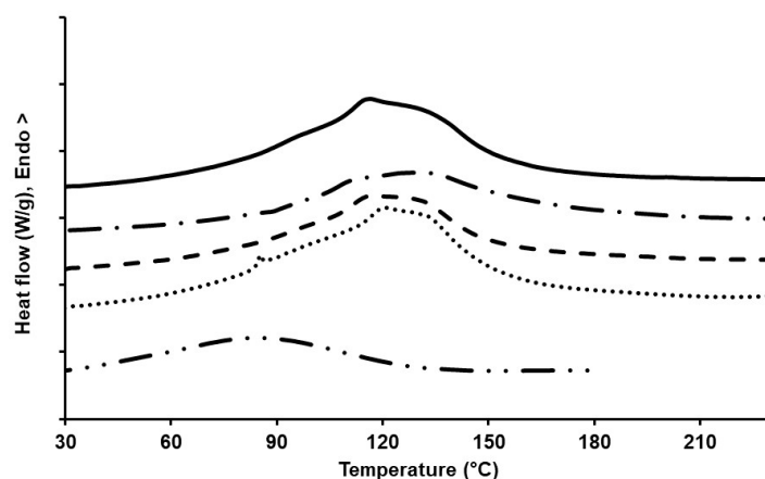
Figure 3. DSC curves of PAN/BL blends with different concentrations of BL and a reference curve for BL; — PAN; —■ PAN-10%wt BL; —■ PAN-20%wt BL; ■■ PAN-30%wt BL; —■ BL.
