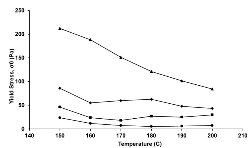
Figure 7. Solution yield stress for PAN and PAN-BL blends as a function of temperature; ●—PAN; ■—PAN-10%wt BL; ◆—PAN-20%wt BL; ▲—PAN-30%wt BL.
