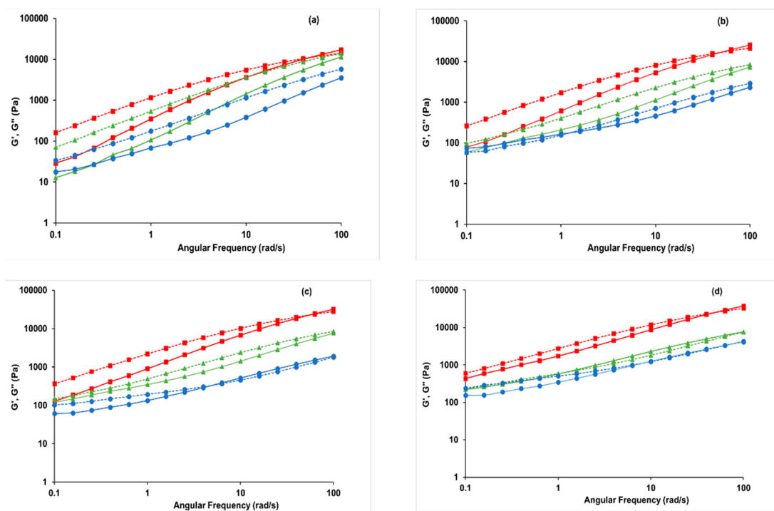
Figure A1. Storage modulus ( G' ) and loss modulus ( G'' ) of (a) PAN; (b) PAN-10%BL; (c) PAN-20%BL; and (d) PAN-30%BL blends as a function of angular frequency at different temperatures. ■—150 °C; ▲—180 °C; ●—200 °C; — G' ; - - - G'' .
