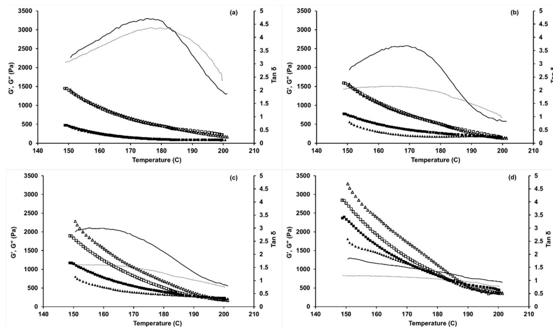
Figure 5. Storage modulus ( G' ), loss modulus ( G'' ) and loss tangent ( \tan \delta ) of (a) PAN; (b) PAN-10%wt BL; (c) PAN-20%wt BL; and (d) PAN-30%wt BL blends as a function of temperature between 150 and 200 °C. \blacktriangle - G' (heating); \blacksquare - G' (cooling); \triangle - G'' (heating); \square - G'' (cooling); \text{—} \tan \delta (heating); \blacksquare \tan \delta (cooling).
