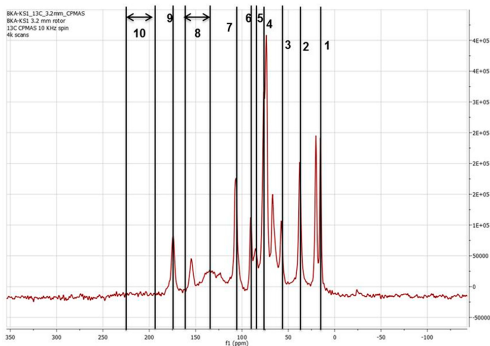
Figure 1. ^{13}\text{C} CP/MAS NMR spectra of butyrate lignin (BL). Description of components/linkages are as follows: 1 → 21–24 ppm ( \text{CH}_3 in acetyl groups in hemicellulose); 2 → 30–40 ppm (alkyl CH & \text{CH}_2 in lignin subunits); 3 → 56 ppm (methoxy groups in lignin G & S units); 4 → 82 ppm ( \text{C}_6 carbon atoms in carbohydrates); 5 → 89 ppm ( \text{C}_4 carbon atoms in carbohydrates); 6 → 105 ppm ( \text{C}_1 carbon atoms in carbohydrates); 7 → 143–167 ppm (unsubstituted olefinic or aromatic C-atoms with OH or RO substituents); 8 → 169–195 ppm (esters & carboxylic acids); 9 → 173 ppm (CH in acetyl groups in hemicellulose); and 10 → 195–225 ppm (carbonyl groups in lignin).
