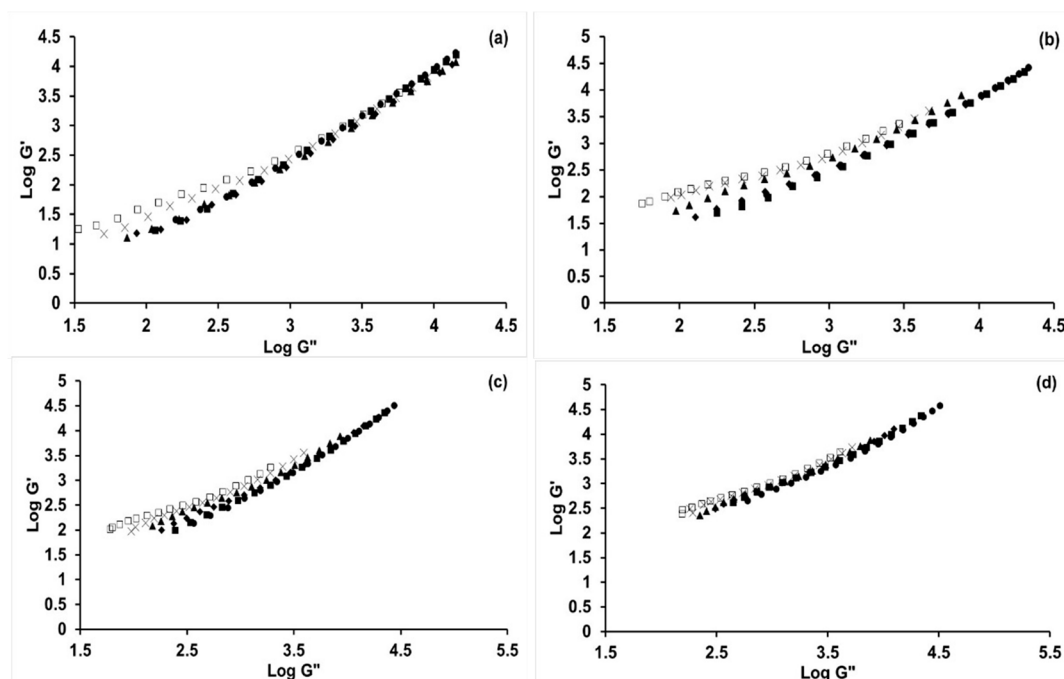
Figure 6. Log-log G'-G'' plot (or Han plot) as a function of temperature for (a) PAN; (b) PAN-10%wt BL; (c) 20%wt BL; and (d) 30%wt BL in [BMIM]Cl; ●—150 °C; ■—160 °C; ◆—170 °C; ▲—180 °C; X—190 °C; □—200 °C.
