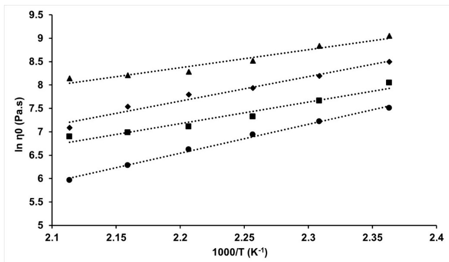
Figure 4. Arrhenius plot for Zero-shear viscosity of PAN and PAN-BL blends as a function of temperature; ●—PAN; ■—PAN-10%wt BL; ◆—PAN-20%wt BL; ▲—PAN-30%wt BL.
