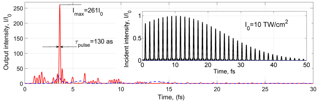
FIG. 3. A single attosecond pulse in the water window spectral range, which is produced as a result of amplification of the attosecond pulse train, shown in the inset, in an active medium of a C^{5+} hydrogenlike x-ray laser. Red solid curve is the amplified z -polarized x-ray signal; the blue dashed curve corresponds to the ASE of y polarization. The length of the active medium is L = 7 mm; the concentration of C^{5+} ions is N_{\text{ion}} = 10^{19} 1/cm 3 .
