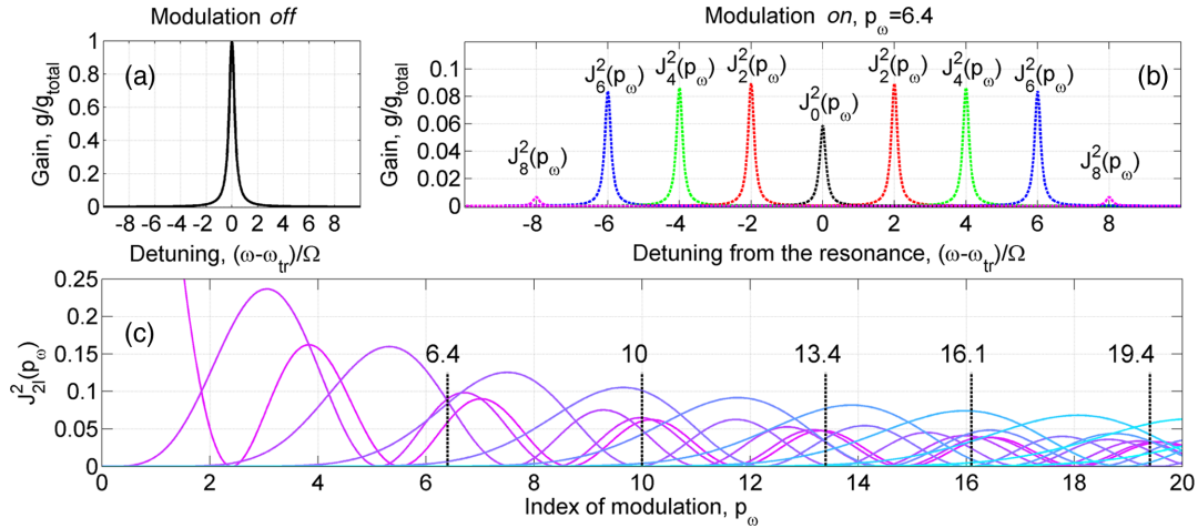
FIG. 1. Frequency dependence of the gain for the incident x-ray field (b) with and (a) without modulating field. In (b), the value of modulation index is p_{\omega} = 6.4 ; black, red, green, blue, and magenta curves correspond to the gain coefficients for 0th, \pm 2 nd, \pm 4 th, \pm 6 th, and \pm 8 th sidebands of the inverted transition. (c) Dependence of the squared Bessel functions of even order (from 0th to 20th order) on the value of modulation index, p_{\omega} . The color reflects the order of Bessel function and is gradually changed from magenta, corresponding to J_0^2(p_{\omega}) , to cyan, which corresponds to J_{20}^2(p_{\omega}) . Vertical dashed lines indicate the values of p_{\omega} , at which the squares of Bessel functions of different orders are comparable to each other [compare with (b)].
