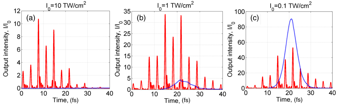
FIG. 2. Time dependence of intensity of an amplified attosecond pulse train of z polarization (red solid curve) and of an ASE of y polarization (blue dashed curve) at the output from an active medium of C^{5+} hydrogenlike x-ray laser. The length of active medium is L = 1 mm, the concentration of C^{5+} ions is N_{\text{ion}} = 10^{19} 1/cm 3 . (a)–(c) correspond to peak intensities of the incident attosecond pulse train I_0 = 10^{13} W/cm 2 , I_0 = 10^{12} W/cm 2 , and I_0 = 10^{11} W/cm 2 , respectively.
