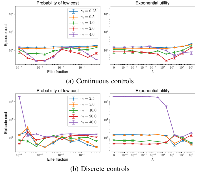
Fig. 4: Varying loss parameter and step size (1000 samples).
