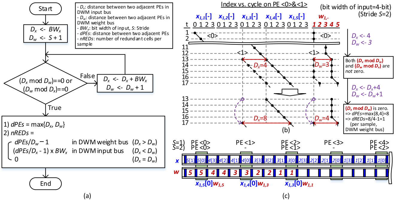
FIGURE 13. The proposed DWM-based cell array for CNN operation: (a) flowchart for finding dPEs (the distance between two adjacent PEs) and nREDs (the number of redundant cells per sample), (b) index vs. cycle chart for BW_x (the bit width of input) = 4 and S (stride) = 2, and (c) the DWM input and weight bus example of S = 1 and 2 ( BW_x = 4 ).
