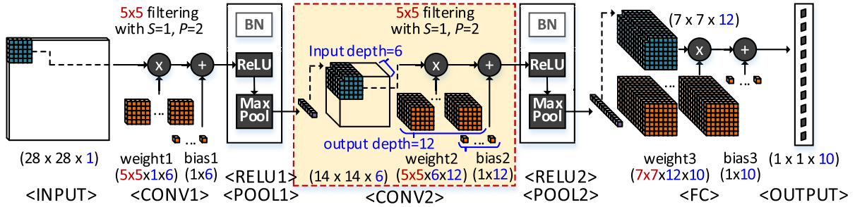
FIGURE 2. A simple convolutional neural network (CNN) with three layers for MNIST ( 28 \times 28 \times 1 ) classification.
