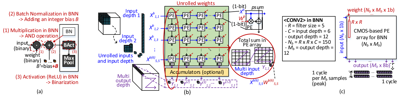
FIGURE 4. (a) Differences of the CNN layer operations between CNN and BNN. (b) The architecture that implements the BNN convolutional layer using 2D PE array. (c) The CONV2 layer example.
