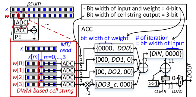
FIGURE 7. The accumulator in PE unit in the DWM-based design.
