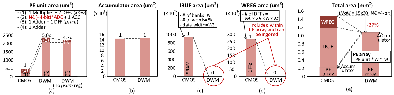
FIGURE 14. Area breakdown of the comparison between the conventional CMOS-based and the proposed DWM-based CNN convolutional layer implementations – (a) PE unit, (b) accumulator, (c) IBUF, (d) WREG, and (e) total (the PE array size N \times M is 15 \times 30 and the bit width of input activations and weights is 4-bit).
