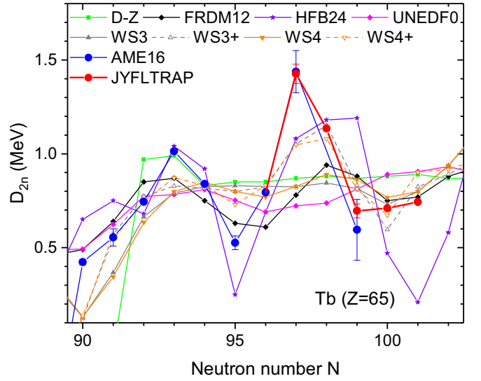
FIG. 14. Experimental D_{2n} values for the Tb isotopic chain, based on AME16 [21] (in blue) and the JYFLTRAP measurements from this work and Ref. [26] (in red), and comparison to various commonly used mass models, such as Duflo-Zuker (D-Z) [72], FRDM12 [22], HFB24 [71], UNEDF0 [84], WS3 [73], WS3+ [74], WS4 [75], and WS4+ [75]. None of these models predict the enhancement seen at N = 97 .
