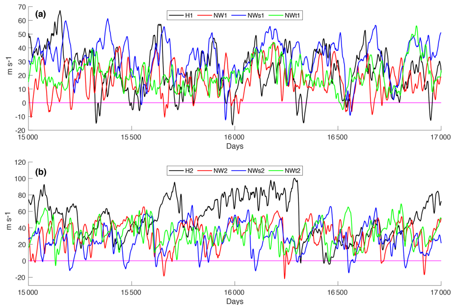
Figure 7. Zonal-mean zonal wind at 10 hPa and 60^\circ \text{N} for H1 and H2 (black), NW1 and NW2 (red), NWs1 and NWs2 (blue), and NWt1 and NWt2 (green) for model runs with wave 1 (a) and wave 2 (b) heating. The data were smoothed with a 10 d filter. The magenta line marks 0 \text{ m s}^{-1} .
