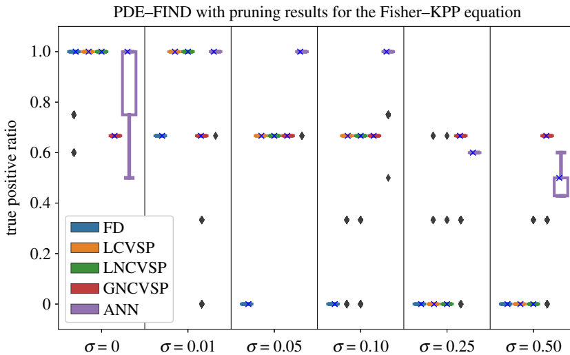
Figure 5. TPR values for the Fisher–KPP equation. We calculated the TPR (see equation (2.12)), for 1000 different training–validation splits. These plots demonstrate the range of TPR values for each case. In each plot, the lower line in the coloured box portion provides the 25% quartile of the data and the upper line denotes the 75% quartile. The ‘ \times ’ on each box plot denotes the median TPR value for that scenario. The lengths of the upper and lower whiskers are 1.5 times the interquartile range, and diamonds denote outlier points. Any plot depicted as a solid horizontal line (e.g. the finite difference computations for \sigma = 0 ) denotes that this value is the majority of the distribution. (Online version in colour.)
