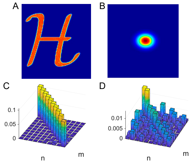
Fig. 3. The reduced idler density matrix in the Schmidt basis. (A) The projected object. (B) The “spot size” corresponding to the HG_{00} mode. (C) The idler's reduced density matrix before the interaction with the object presented in Hermite–Gauss basis modes, given by Eq. 9. (D) The change in the reduced density matrix of the idler due to the interaction with the object given by Eq. 10.
