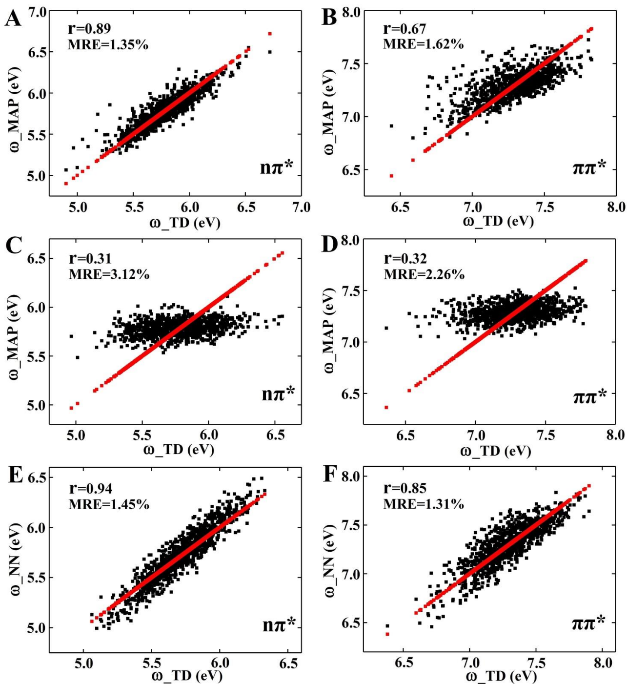
Fig. S3. (A) Correlation plots of n\pi^* transition energies by TDDFT ( \omega_{\text{TD}} ) and map method ( \omega_{\text{MAP}} ). 1 (B) Same as (a) but for the \pi\pi^* transition. (C) Comparison of n\pi^* transition energies by TDDFT ( \omega_{\text{TD}} ) and map method ( \omega_{\text{MAP}} ) 1 which fitted by different data sets. (D) Same as (C) but for the \pi\pi^* transition. (E) Comparison of n\pi^* transition energies by TDDFT ( \omega_{\text{TD}} ) and neural network ( \omega_{\text{NN}} ). (F) Same as (E) but for the \pi\pi^* transition. The red lines/dots on the figures represent the transition energies ( \omega_{\text{TD}} ) of NMA calculated by TDDFT which performed at the (B3LYP/6-31G(d,p)) level.
