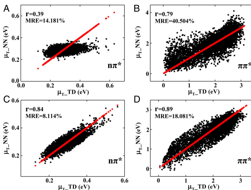
Fig. 3. NN prediction of the NMA transition dipole moment. (A) Correlation plots of n\pi^* transition dipole moment by TDDFT ( \mu_{\text{T-DT}} ) and NN ( \mu_{\text{T-NN}} ) using descriptors of CM on test data. (B) Same as A but for the \pi\pi^* transition. (C) Comparison of n\pi^* transition dipole moment by TDDFT ( \mu_{\text{T-DT}} ) and NN ( \mu_{\text{T-NN}} ) using descriptors of CM based on NPA charge ( \text{CM}_Q ) on test data. (D) Same as C but for the \pi\pi^* transition. The red lines/dots represent the \mu_{\text{T-DT}} of NMA calculated by TDDFT at the PBE0/cc-pvdz level.
