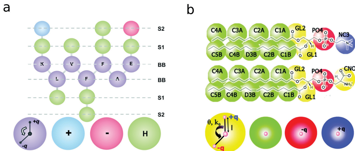
Fig. 3 (a) Peptide – Water-Explicit Polarizable PROtein Model (WEPPROM) reproduced from Sahoo et al. 99 (b) Membrane – Water-Explicit Polarizable MEMbrane (WEPMEM) model reproduced from Ganesan et al. 100 with permission from the PCCP Owner Societies. The partial charges on peptide backbone (violet) and polarizable beads (yellow) of lipids generate explicit structural polarization and provide directionality to dipolar interactions that can result in structural transitions.
