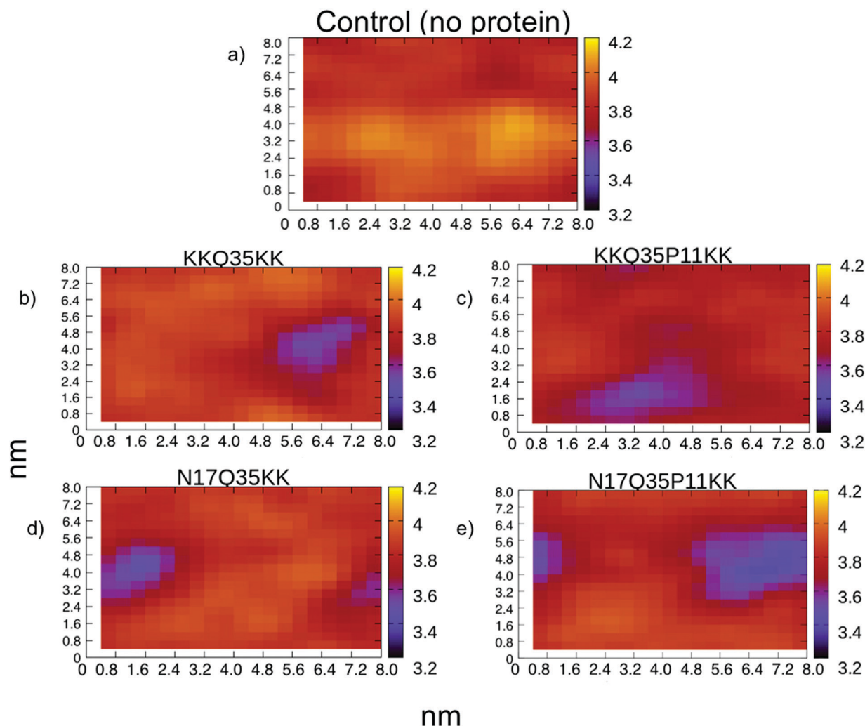
Fig. 6 Thickness of membrane of control system and different peptide variants. Reprinted with permission from A. Nagarajan, S. Jawahery and S. Matysiak, J. Phys. Chem. B , 2014, 118 , 6368–6379.
