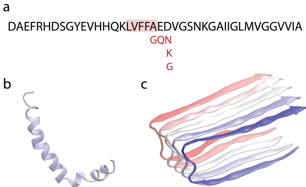
Fig. 2 (a) Amino acids in A \beta 1–42 peptide. The red shaded region represents the central hydrophobic core and the characters in red are some of the familial mutants. (b) In-solution structure of a single monomer in apolar micro-environment (pdb: 1IYT). (c) A representative structure of A \beta oligomer (pdb: 2BEG) in solution. The aggregate is colored to distinguish peptide chains. A \beta oligomers are highly dynamic and can have different structure depending on local environmental changes.
