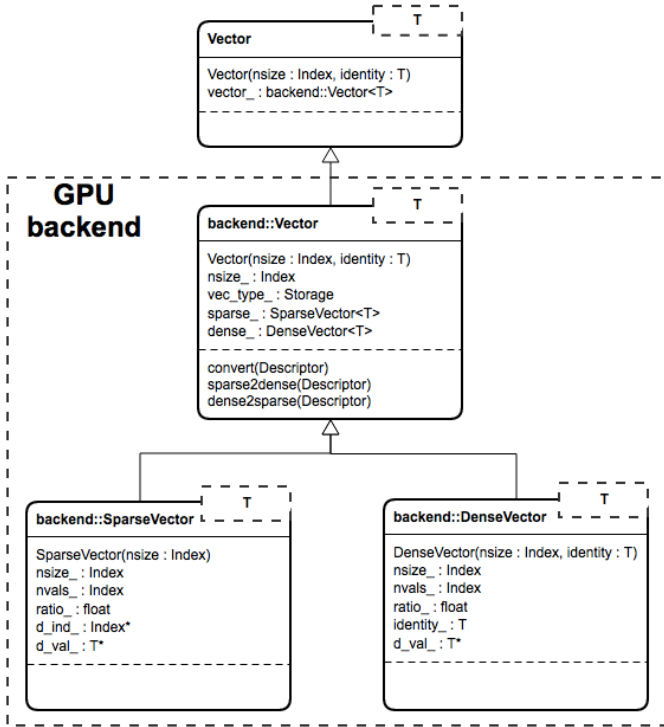
Fig. 3: GraphBLAST Vector UML diagram.
