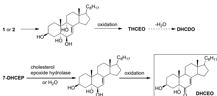
Figure 10. Mechanisms of the formation of 7-DHC-derived oxysterols in solution (A,B) and in biological systems (C). (A) Primary pathways of 7-DHC autooxidation in organic solution at 37 °C; (B) 7-DHC autooxidation in the presence of \alpha -tocopherol (only loss of the H-9 pathway is shown); (C) metabolism of primary 7-DHC oxysterols in cells. Compounds highlighted in the rectangle are potential electrophiles.
