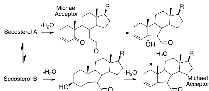
Figure 13. Dehydration of secosterols gives a complex mixture of electrophiles, including two Michael acceptors.
