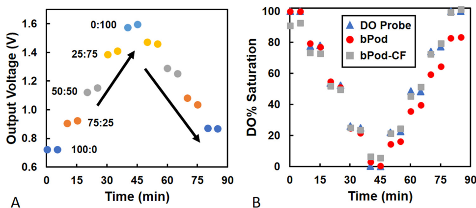
Fig. 6. Electrochemical response of untethered bPod (w/ battery) in the 10-L bioreactor setup. Gas input is alternated every 10 minutes ( O_2:N_2 - 100:0, 75:25 50:50, 25:75, 0:100) over a 1.5-h period and DO is measured at a 5-minute interval. (A) Output voltage from the bPod recorded at 10 s. (B) Comparison of the DO% saturation of the inline DO probe (blue, triangle), bPod (red, circle), and corrected bPod (bPod-CF) (gray, square).
