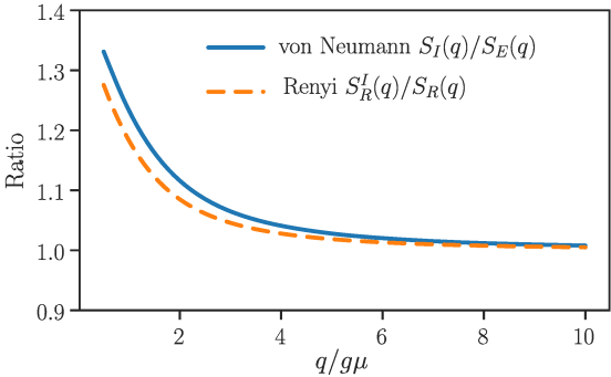
FIG. 1. Ratios of entropy densities at a given magnitude of the transverse momentum \mathfrak{q}=g\mu . S_{I2}\delta\mathfrak{q}^2\mathfrak{p} is the von Neumann entropy density of ignorance and S_{E}\delta\mathfrak{q} \mathfrak{p} is the corresponding entanglement entropy density. The same for Renyi entropy densities.
