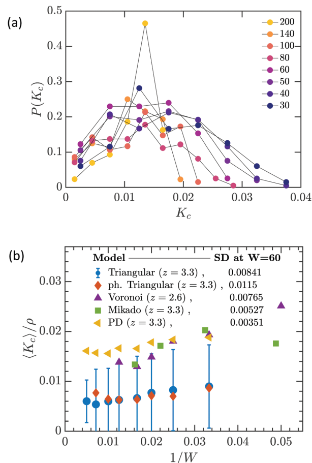
Fig. 7 (a) The distributions of shear modulus discontinuity K_c for triangular networks with z = 3.3 and different system sizes as specified in the legend. (b) Shear modulus discontinuity K_c versus inverse system size 1/W , for various 2D network models as specified in the legend (for Mikado model we used square root of present nodes in the network as W ). The data are normalized with the length density \rho for every model. The standard deviations are only shown for the triangular network, though the standard deviation at W = 60 for every model is shown in the legend.
