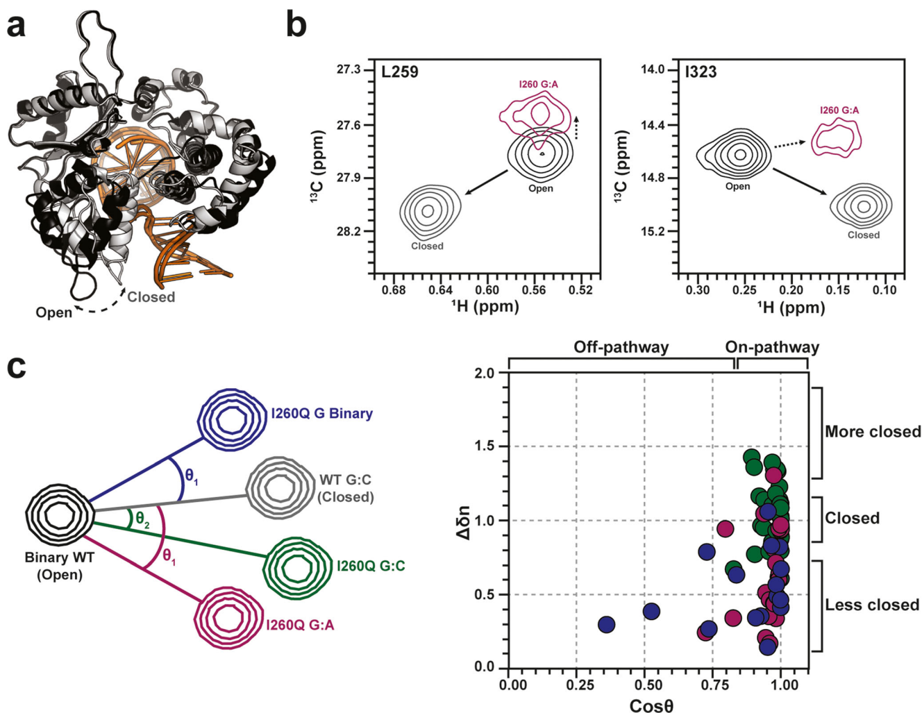
Fig. 6 a X-ray crystal structures of open (black) and closed (gray) pol β. DNA molecules are shown in orange shades. b NMR chemical shift signatures of the open (black, WT without nucleotide), closed (gray, WT with matched nucleotide), and “off-pathway” (purple, I260Q mutant with mismatched nucleotide) structural states of pol β. c Schematic representation of chemical shift vector analysis reported by Liptak et al., accounting for various degrees of enzymatic closure around matched and mismatched nucleotides in WT and I260Q mutant pol β. WT pol β adopts its native, closed structure upon matched dNTP binding (black,
