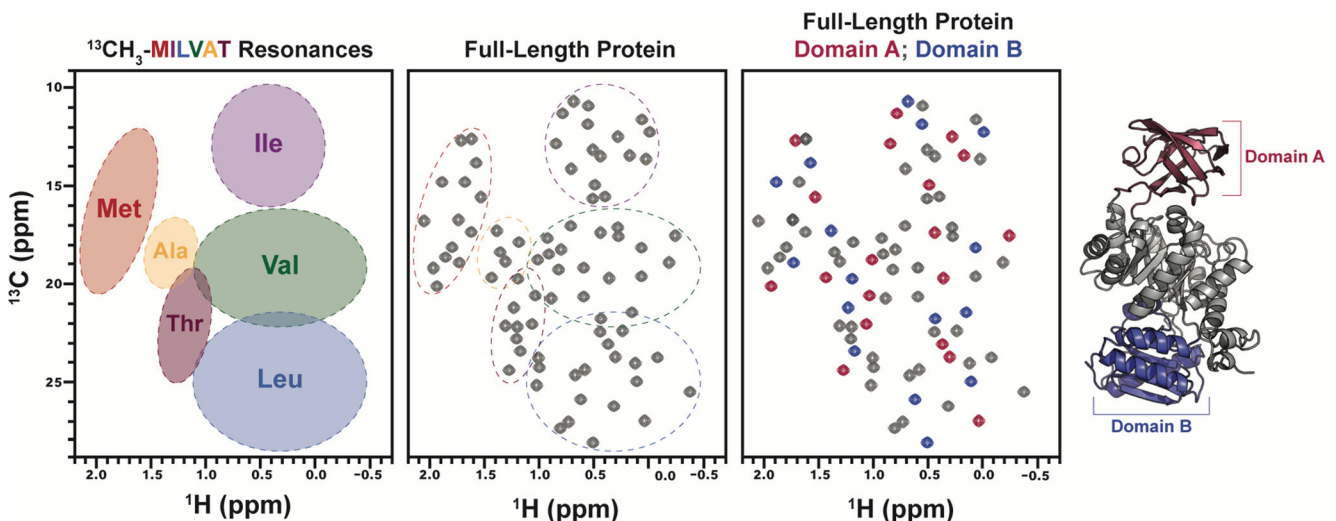
Fig. 5 ^{13}\text{CH}_3 -labeling of Met-Ile-Leu-Val-Ala-Thr residues can deconvolute NMR spectra of large proteins and effectively resolve amino acid types by chemical shift. NMR studies of small subdomains within larger proteins and complexes remain popular, and the ability to
