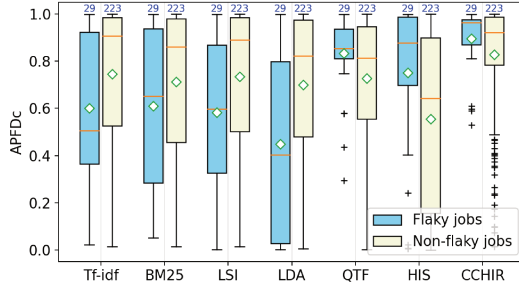
Figure 5: Comparing different techniques on flaky/non-flaky jobs
