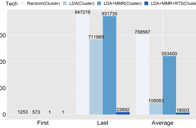
Figure 5: Test case execution
