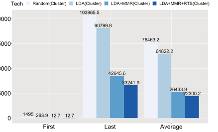
Figure 6: Test execution time
