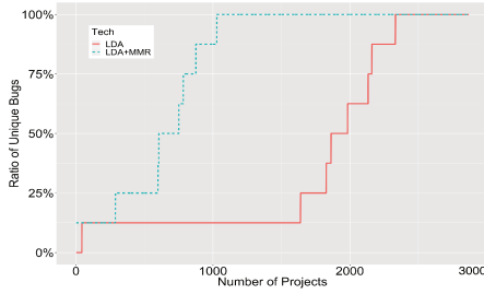
Figure 13: Accumulated bugs detected
