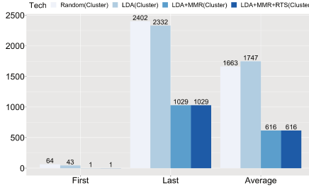
Figure 4: Client project execution
