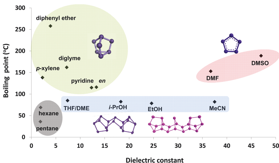
Scheme 2. Correlation between the Solvent's Characteristics and the Major Polyphosphide Products Observed in the Reactions between P_{red} and KOEt
