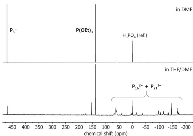
Figure 1. ^{31}\text{P}\{^1\text{H}\} NMR spectra of the reaction mixtures obtained by the activation of \text{P}_{\text{red}} with KOEt in refluxing DMF (top) and in refluxing THF/DME (bottom).
