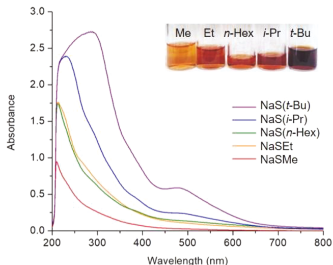
Figure 2. Optical absorption spectra of soluble polyphosphide products obtained in the 24 h reactions with thiolate activators in THF/DME (1:1 v/v). The inset shows the appearance of resulting solutions.
