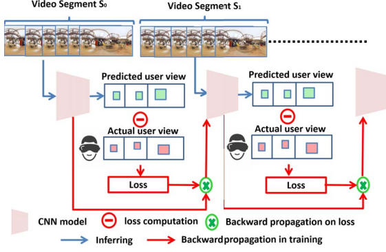
Figure 2: CNN-based viewport prediction workflow.
