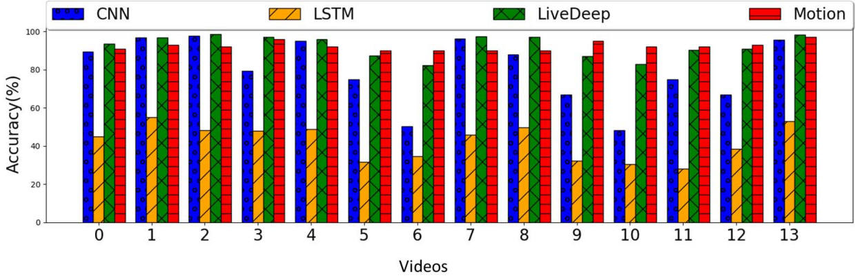
Figure 4: Overall prediction accuracy (Epoch=10,VGG13) with the comparison among the four methods.
