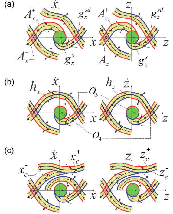
FIG. 13. Schematic diagrams for (x, \dot{x}) and (z, \dot{z}) projections of vector flow (8), bounded by the trajectories of 2D auxiliary systems A_x^\pm and A_z^\pm ( A_x^- and A_z^- ) depicted in red (blue). (a). Typical arrangement of vector flow (8) corresponding to region I (see Fig. 2). The unstable manifolds of the auxiliary systems' saddles form trapping regions ("rivers") that attract the trajectories of system (8) and guide them into trapping disks g_x^s and g_z^s (green). (b) Arrangement of vector flow (8) from region II which allows the formation of the homoclinic orbit h_x ( h_z ) of saddle focus O_3 ( O_4 ). Note that the saddle focus O_3 lies inside saddle cell g_x^{sd} (pink diamond-shaped region) in the (x, \dot{x}) projection and inside stable region g_z^s (green disk) in the (z, \dot{z}) projection, representing its focus part. Saddle-focus point O_4 is symmetric to O_3 , with its x ( z ) coordinate inside g_x^s ( g_z^s ). (c) Region III. The auxiliary systems are bistable, each having a stable fixed point and a stable limit cycle. These limit cycles x_c^+ and x_c^- ( z_c^+ and z_c^- ) form a trapping river (the upper horizontal strip) which contains rotatory trajectories of (8). Trapping disks g_x^s and g_z^s (green) contain oscillatory trajectories of (8).
