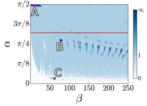
FIG. 4. Regular and chaotic phase shift dynamics of system (8) evaluated numerically as a function of parameters \alpha and \beta . The color coding corresponds to the period of a limit cycle. White regions correspond to fixed points with a zero winding number; light blue regions correspond to a winding number of 1 (period-1 limit cycles); dark blue regions correspond to chaotic orbits with infinitely large winding numbers. Sample points A, with (\beta, \alpha) = (10, 397\pi/800) ; B, with (\beta, \alpha) = (78.125, 437\pi/1600) ; and C, with (\beta, \alpha) = (61.5625, 27\pi/800) , correspond to chaotic mixed-mode-mixed-mode, rotating-rotating, and oscillating-rotating phase shift regimes, respectively (see Figs. 5–7). The red horizontal line corresponds to the line \omega = 1 - a in Fig. 3. The region under the red line is region II, where homoclinic bifurcations give birth to chaos. Other parameters are as in Fig. 3.
