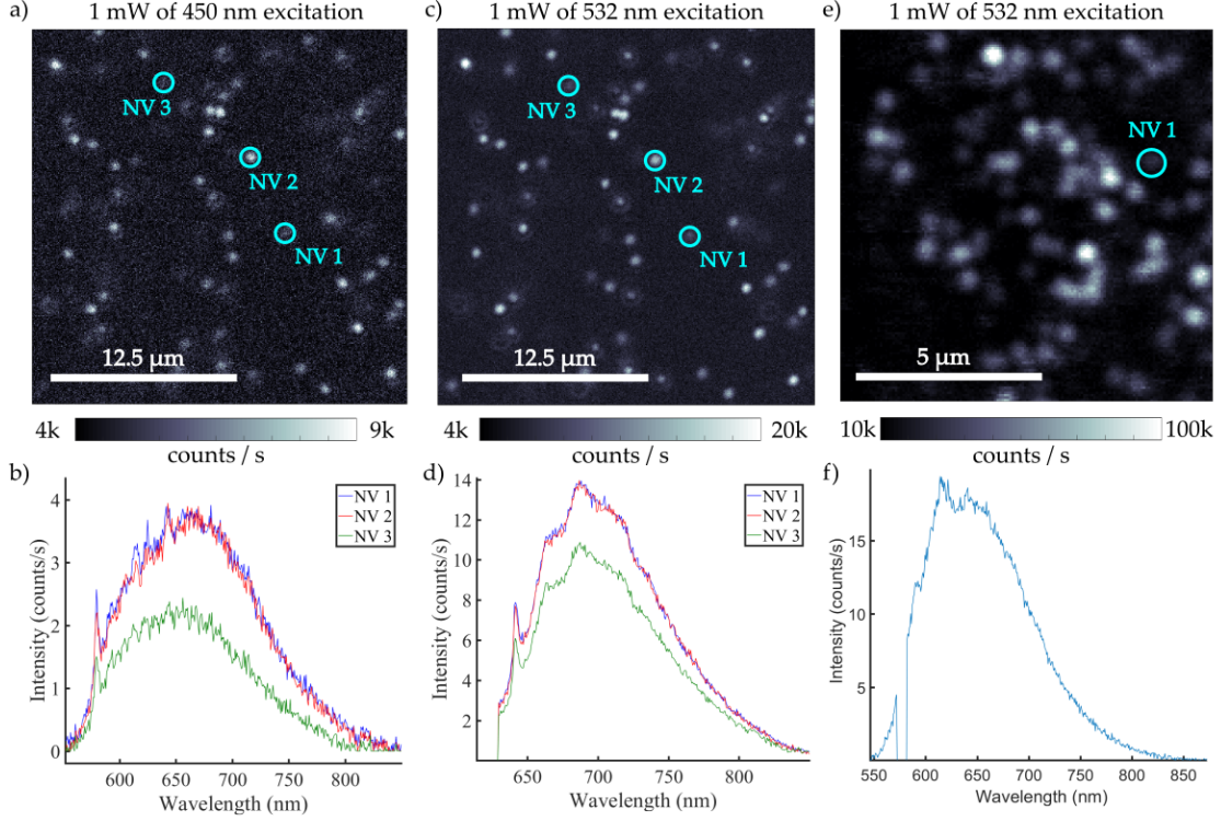
FIG. S7: (a,b) Confocal scan and spectra of 3 NVs in sample B taken with 450 nm excitation. (c,d) Confocal scan and spectra of same 3 NVs in sample B taken with 532 nm excitation. (e,f) Confocal scan and spectra of NV^0 from a reference sample taken with 532 nm excitation.
