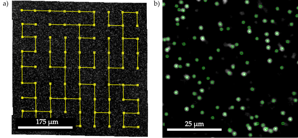
FIG. S3: (a) 350 \mu\text{m} \times 350 \mu\text{m} stitched large-area scan after anneal #12 showing the MST graph. (b) A 50 \mu\text{m} \times 50 \mu\text{m} scan showing \text{NV}^- position detection via CHT algorithm.
