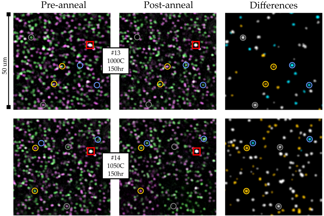
Figure 2. A sequence of subareas of the “large-area scan” confocal images showing \text{NV}^- changes. Green and magenta indicate the two sets of distinguishable \text{NV}^- orientations. Two examples each of appearances, disappearances and re-orientations are indicated by blue, grey and yellow circles, respectively. The red square marks a persistent defect used for image alignment.
