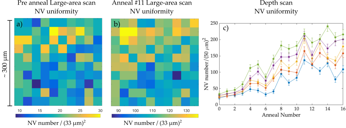
FIG. S4: (a) Variation in \text{NV}^- density across large-area scan region pre-anneal. (b) Variation in \text{NV}^- density across large-area scan region after anneal #11. (c) Variation in \text{NV}^- density across 5 sampled regions at a depth of 240 \mu\text{m} , as a function of anneal number. Each location is denoted by a different color. Error bars indicate one-sigma uncertainty for a Poisson distribution.
