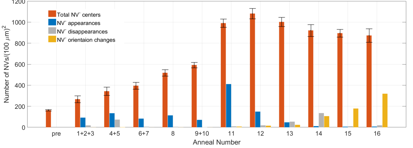
Figure 3. Total NV - density and observed changes obtained from the large-area scans ( \approx 350 \times 350 \mu\text{m}^2 ) of sample B after every anneal. Several anneals are combined due to an inability to accurately match a significant portion of the scan area in the intermediate scans. For combined anneals, comparisons are made before and after the first and last anneal. Error bars represent uncertainty due to automation errors and differences in scan area between datasets [15]. Note the significant increase in annealing time which occurs at anneal 11.
