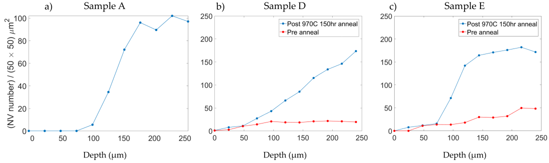
FIG. S6: (a) Number of NVs in Sample A as a function of depth after 1100°C anneal. (b) Sample D pre and post anneal. (c) Sample E pre and post anneal.
