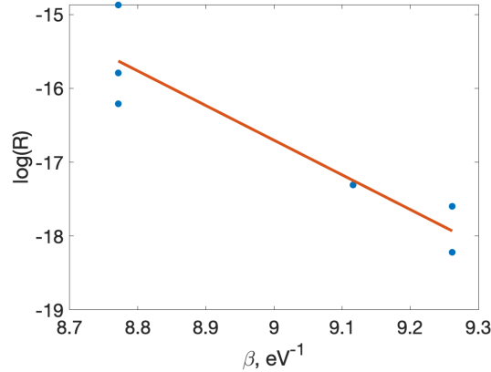
FIG. S8: Log of the reorientation rate as a function of \beta = (k_B T)^{-1}
