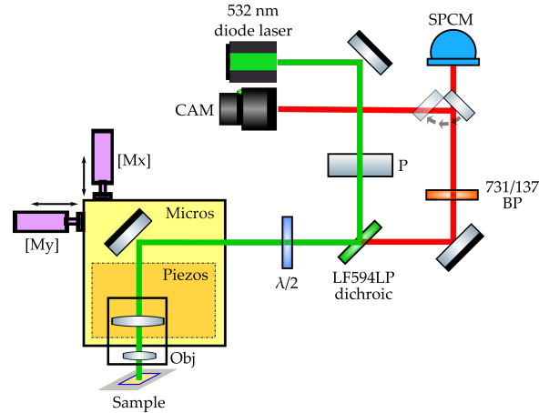
FIG. S1: Schematic of the microscope setup
