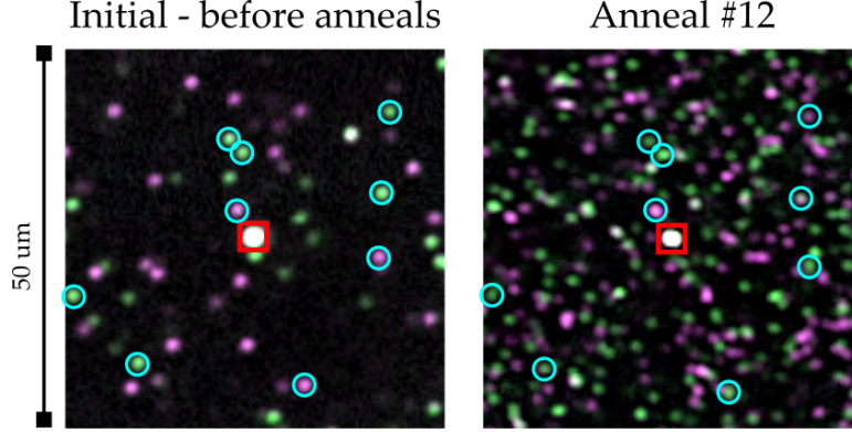
FIG. S2: Crop ( 50\text{ }\mu\text{m} \times 50\text{ }\mu\text{m} ) of large-area scan data from Sample B showing the increase in \text{NV}^- density from initial (no-anneals) state to post anneal #12 (maximum \text{NV}^- density). The blue circles mark NVs retained through the anneals. The red square marks a persistent defect used for image registration.
