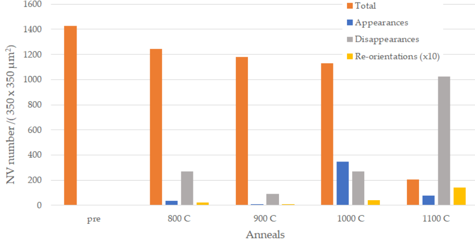
FIG. S5: Large-area scan data from sample A at a depth of 96 \mu\text{m} , as a function of anneal temperature. The ramp and hold times were each 2 hours for every anneal. The appearances and disappearances were manually counted in this dataset.
