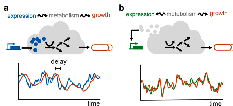
Figure 3. Following metabolic fluctuations in time. Individual cells display gene expression and growth rates that vary strongly in time, in a correlated fashion, by at least two different mechanisms: (a) Fluctuations in the expression of limiting metabolic enzymes lead to metabolic fluxes that vary in time, which in turn cause delayed growth rate fluctuations. Adapted with permission from ref 102 . Copyright 2014 Springer Nature. (b) Expression itself is also affected by metabolic fluctuations, possibly mediated by varying levels of amino acids or ATP. This mechanism also generates correlations in expression and growth fluctuations but without the time delays seen in panel a. Adapted with permission from ref 124 . Copyright 2018 Elsevier.
