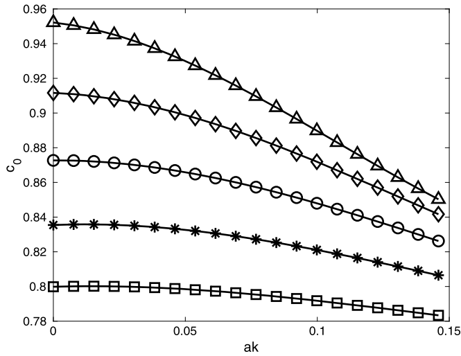
Fig. 3. Phase velocity of the traveling-wave solutions as a function of the wave steepness, c_0 increases as \Omega increases. This feature was observed by Kharif and Abid [9] within the framework of a fully nonlinear, generalized vor-Whitham equation, whereas the profiles shown in Fig. 1 are weakly nonlinear.
