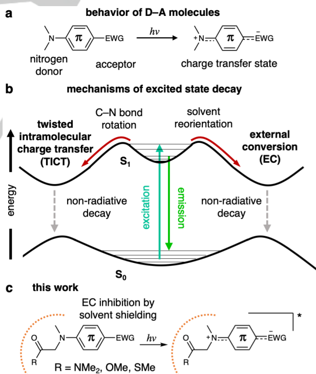
Figure 1. Proposed \beta -carbonyl donor attenuates solvent-mediated excited state decay. a) Common scaffold of D–A molecules. b) Established mechanisms of thermal, non-radiative excited state decay. c) Proposed role of \beta -carbonyl based donors to attenuates solvent-mediated excited state decay. (EWG: electron withdrawing group).
