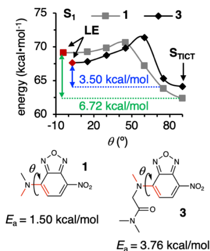
Figure 3. TICT inhibition reduces excited-state decay with \beta -carbonyl functionalization. Potential energy surface scan for rotation (indicated by the red arrow) about highlighted bond in 1 and 3 . Red markers correspond to the calculated LE geometry.
