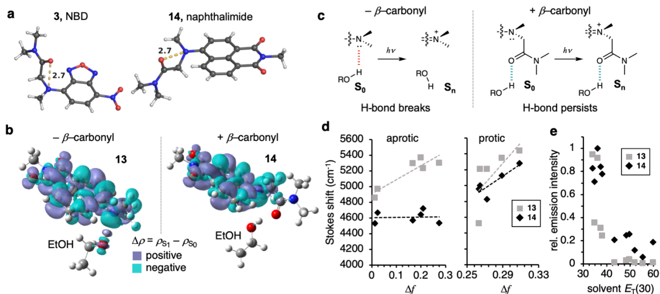
Figure 4. Solvent shielding collectively reduce environmental sensitivity with β-carbonyl functionalization. a) Crystal structures of 3 and 14 . Labeled distances (Å) correspond to yellow dashes. b) Electron density difference during excitation calculated for 13 and 14 with an explicit ethanol solvent molecule geometrically optimized about the donating group. c) Broken H-bond upon excitation of 13 , but not 14 . d) Lippert-Mataga plot of 13 and 14 in both aprotic (dimethylformamide, toluene, 1,4-dioxane, tetrahydrofuran, ethyl acetate, methyl t -butyl ether) and protic (methanol, ethanol, i -propanol, n -butanol, 2,2,2-trifluoroethanol) solvents. e) Relative emission intensity plotted against solvent E_T(30) for the solvents characterized.
