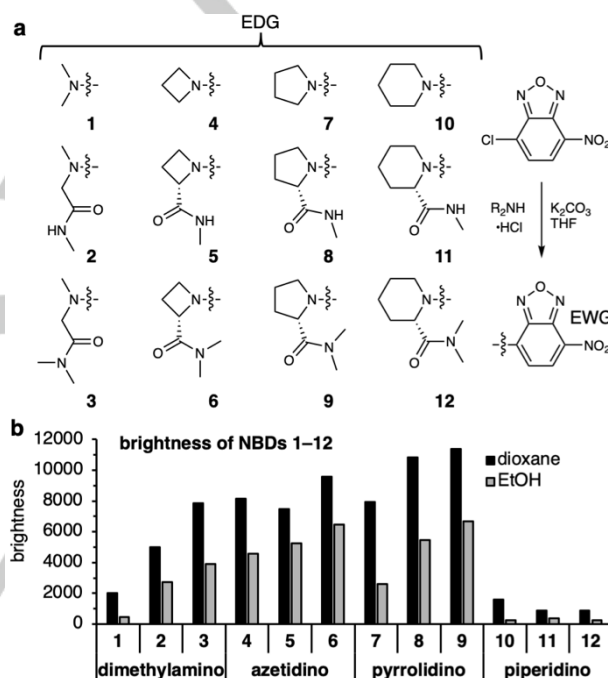
Figure 2. \beta -carbonyl donors enable enhanced photophysical properties in a model D–A fluorophore, NBD. a) The amide based \beta -carbonyl NBD library. b) Brightness of NBDs 1–12 as determined in ethanol and 1,4-dioxane. (brightness = \Phi_f \cdot \epsilon ). Fluorescence quantum yields were measured relative to a fluorescein standard ( \Phi_{std} = 0.79 in 0.1 M aqueous NaOH).
