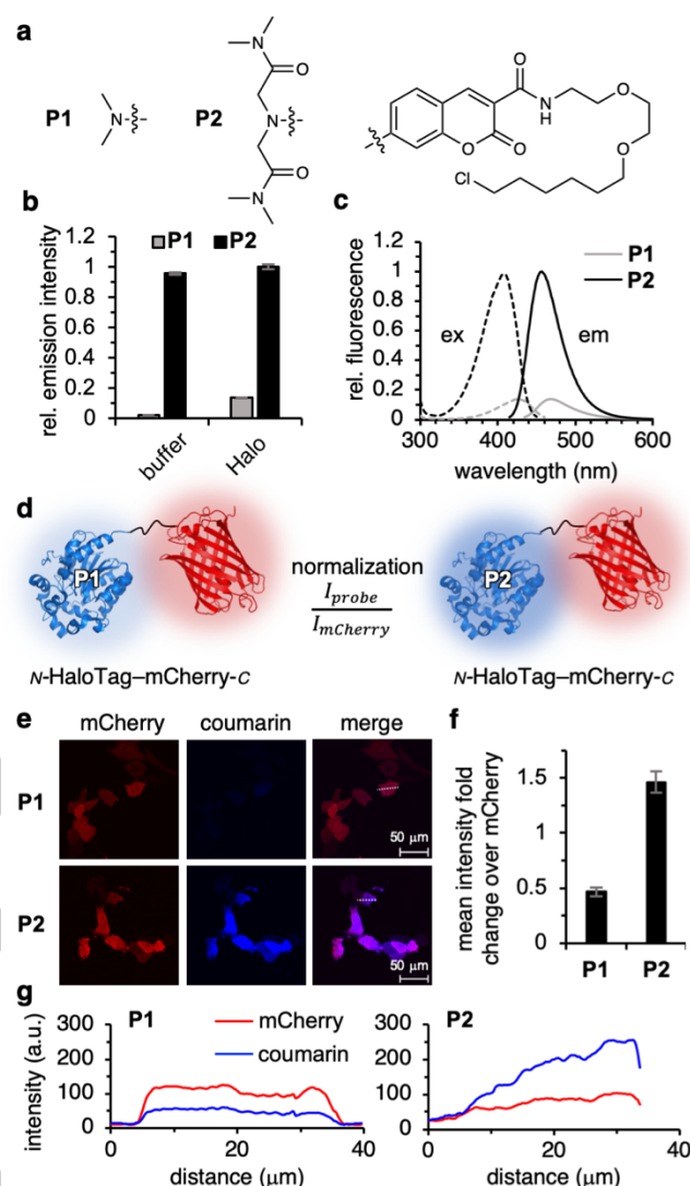
Figure 6. Improved brightness of a bis- \beta -amide coumarinyl probe in cellular imaging. a) Structures of P1 and P2 . b) In vitro characterization of P1 and P2 (5 \mu\text{M} ) fluorescence intensity in 50 mM tris-HCl buffer (100 mM NaCl, pH 7.5) and in conjugation with purified HaloTag protein (25 \mu\text{M} ) in tris buffer (standard error, n = 3 ). c) Excitation (dashed lines) and emission spectra (solid lines) of P1 (grey) and P2 (black) upon conjugation with purified HaloTag protein in tris-HCl buffer. d) Normalization strategy to account for expression level in cell imaging analysis of P1 and P2 by ratio of mean pixel intensity of probe ( I_{\text{probe}} ) to that of the mCherry ( I_{\text{mCherry}} ) domain in a transiently expressed N-HaloTag-mCherry-C fusion protein. e) Live-cell confocal microscopy of HeLa cells transiently expressing an N-HaloTag-mCherry-C fusion protein for 24 h in the presence of P1 or P2 (0.5 \mu\text{M} ) after a single wash. f) Quantified mean pixel intensity fold-change of probe signal relative to that of mCherry (standard error, n = 3 ). g) Intensity profiles of mCherry (red) and probe (blue) signal corresponding to the marked cross sections (white dotted lines) in panel f.
