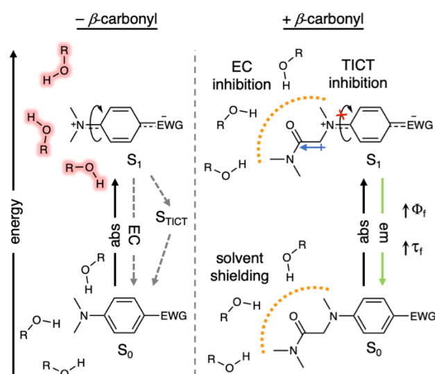
Figure 7. Proposed mechanism governing the enhancement of photophysical behavior in D-A fluorophores with \beta -carbonyl functionalization. Non-radiative decay mechanisms indicated by grey, dashed arrows.
