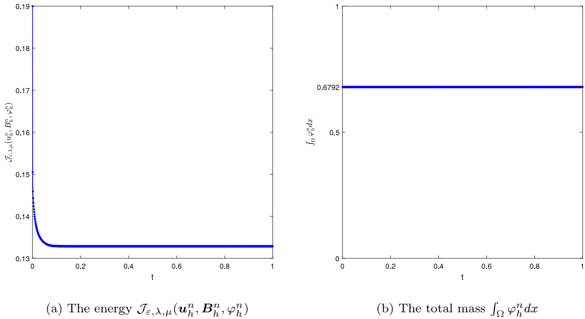
Fig. 1. The energy dissipation and mass conservation.
