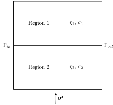
Fig. 4. The region of two-phase Hartmann flows.
