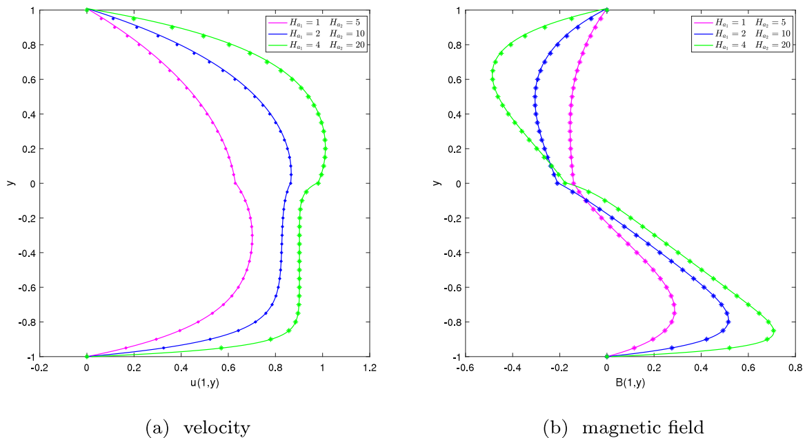
Fig. 7. Horizontal component of velocity and magnetic field along x = 1 for different Hartmann numbers, computed (points) and theoretical (lines).
