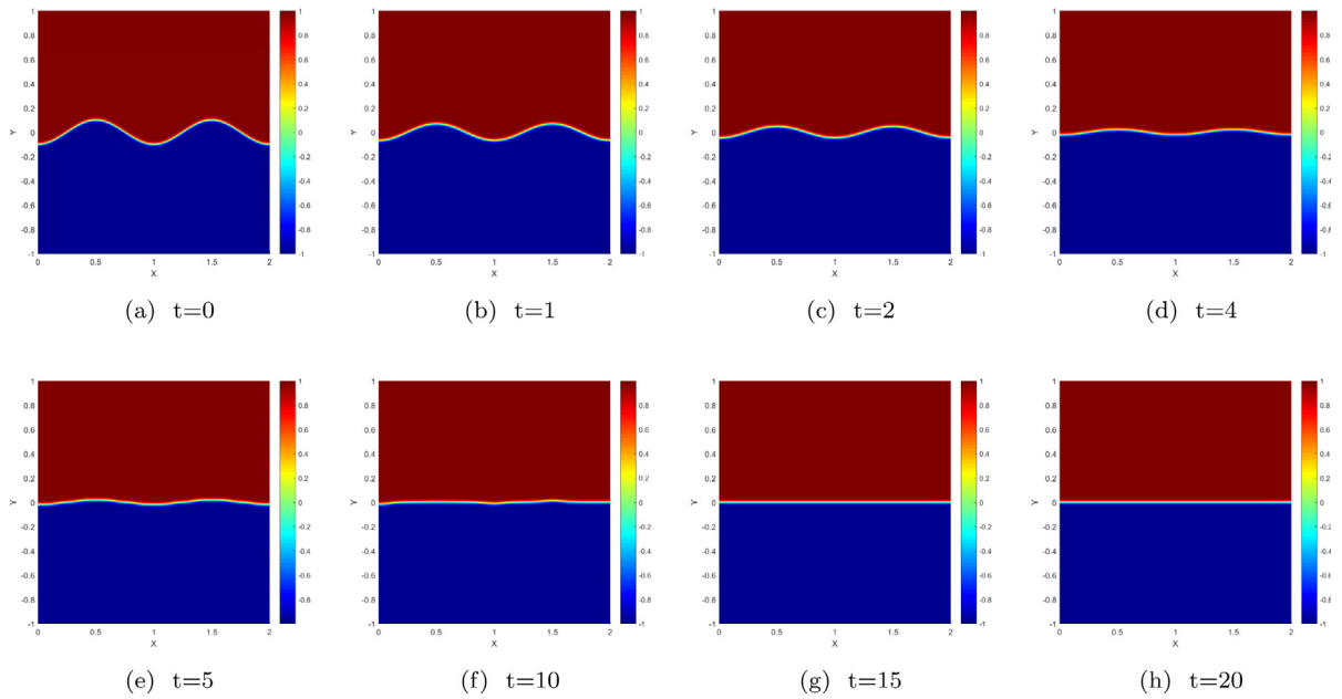
Fig. 3. Phase field \varphi at different time t for \alpha = 0.05 .
