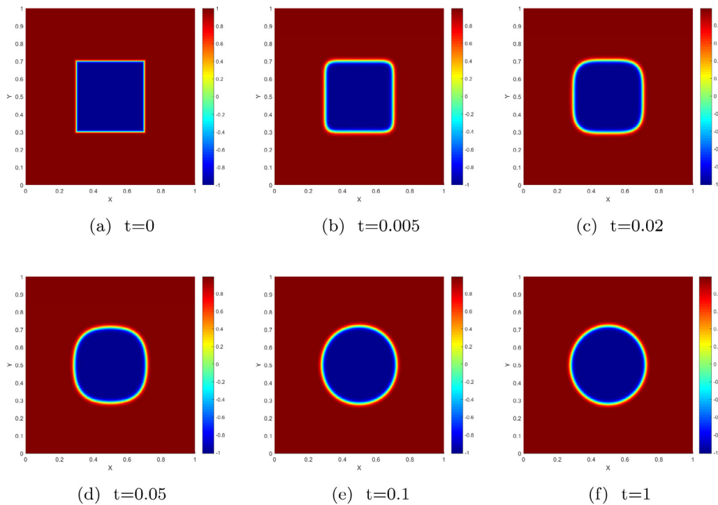
Fig. 2. Phase field \varphi at different time t .
