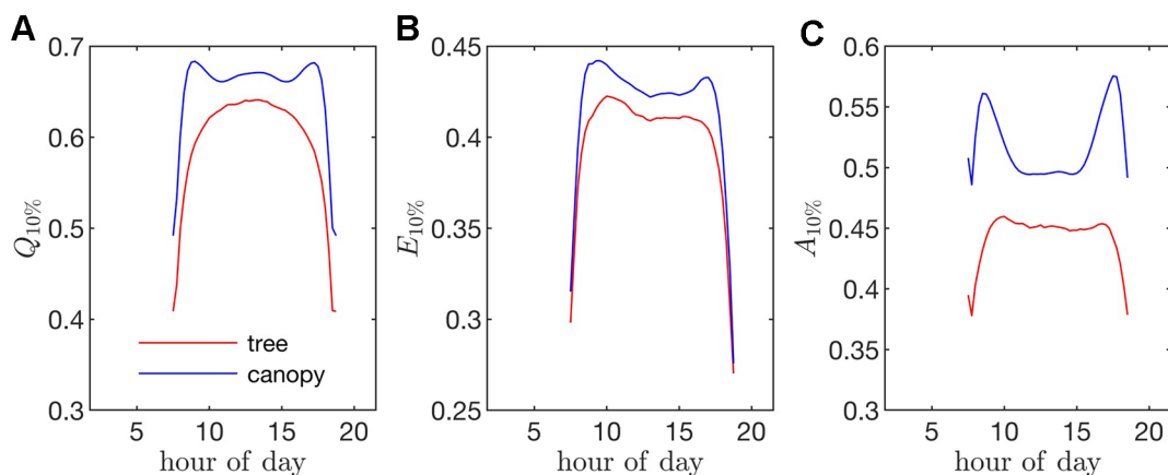
FIGURE 10 | Fraction of the instantaneous flux due to the top 10% of all leaves (i.e., fraction of flux contained in the 90th percentile of leaves) for fluxes of (A) absorbed photon flux Q_{10\%} , (B) transpiration rate E_{10\%} , and (C) net photosynthesis A_{10\%} . (For example, a Q_{10\%} value of 0.75 would mean that only 10% of the leaves were responsible for 75% of the total absorbed PAR for the whole tree/canopy).
