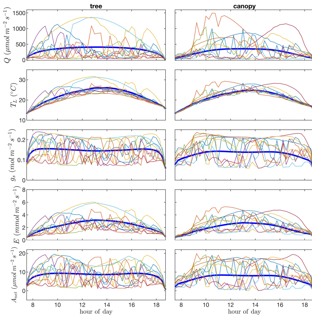
FIGURE 11 | Time-series or “trajectories” for 10 randomly selected leaves of photosynthetic photon flux density Q , leaf temperature T_L , stomatal conductance g_s , transpiration flux E , and net photosynthetic flux A . Each line/color represents the time series of a single leaf. Thick blue lines give the average over all leaves in the tree canopy.
