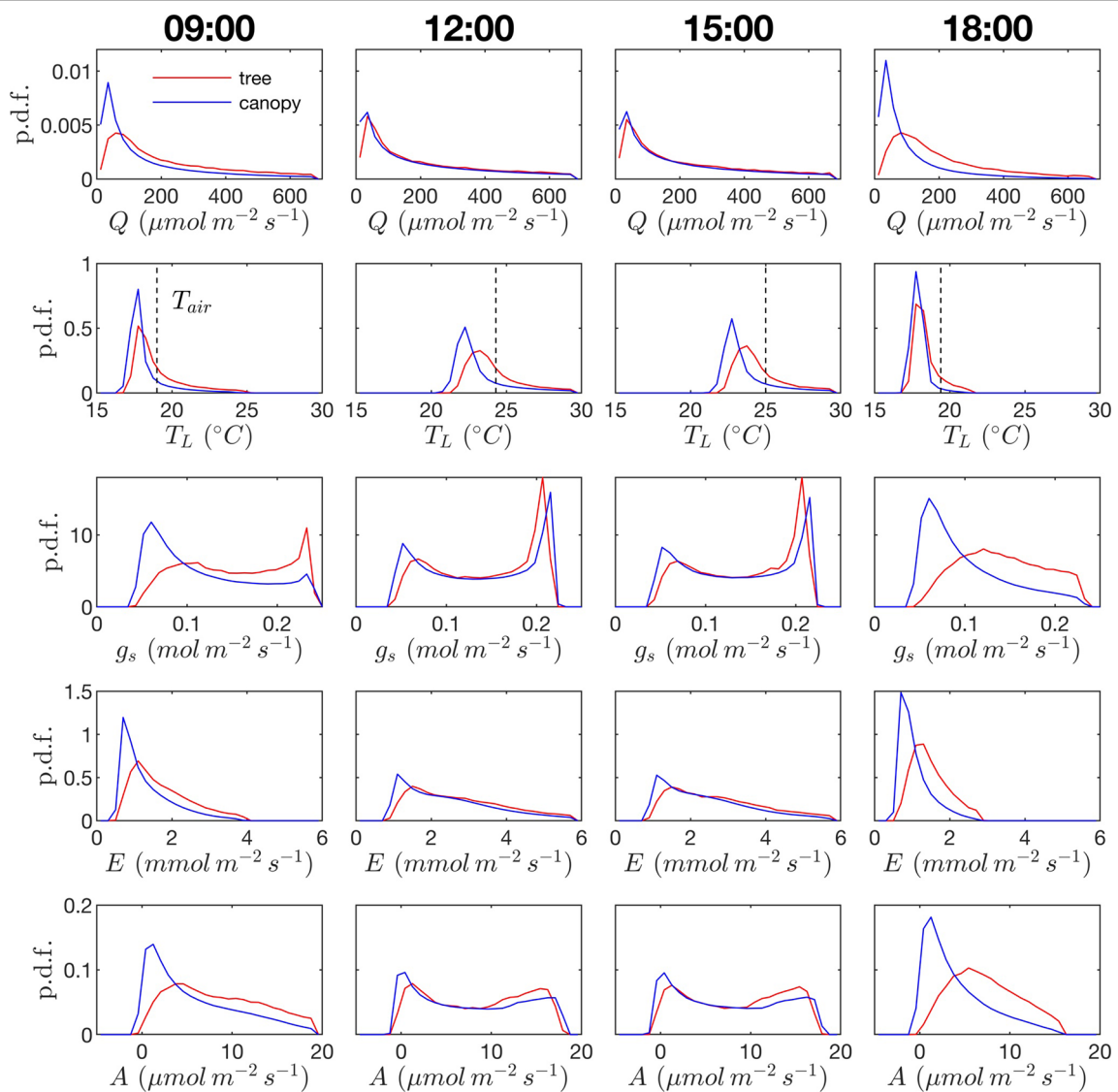
FIGURE 8 | Probability density function (p.d.f.) across all leaves in the canopy for photosynthetic photon flux density Q , leaf temperature T_L (ambient temperature given by dashed vertical line), stomatal conductance to water vapor g_s , transpiration rate E , and net rate of photosynthesis A . Columns correspond to different times of the day. Red lines correspond to the isolated tree case; blue lines correspond to the dense canopy case
