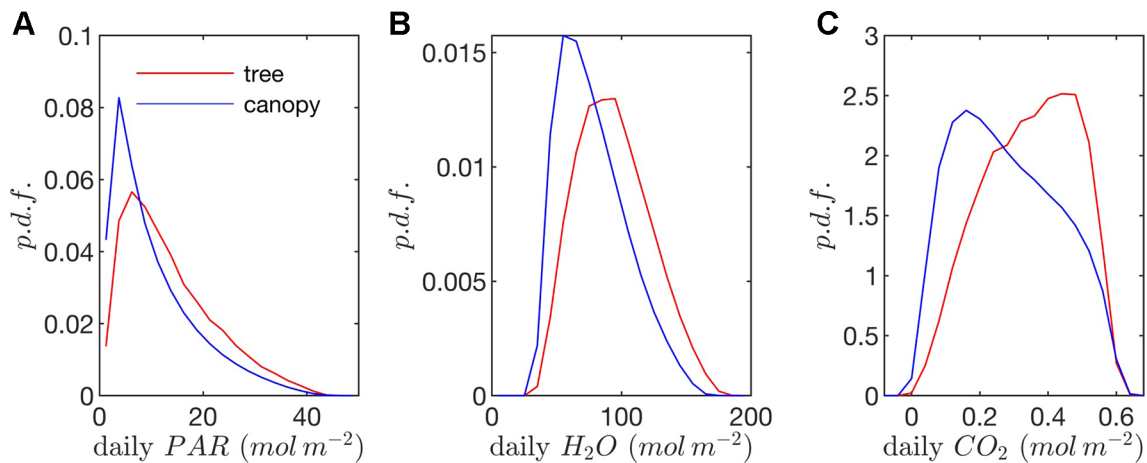
FIGURE 9 | Probability density functions (p.d.f.s) of daily (A) absorbed photosynthetic photons, (B) transpired water, and (C) net \text{CO}_2 exchange (all per unit leaf area).
