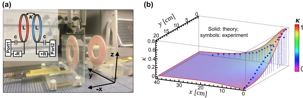
FIG. 10. (a) Measurement setup for the coupling strength between two coils. (b) Coupling strength as a function of distance (x, y) ; theoretical and experimental results are denoted by the isosurface and symbols.
