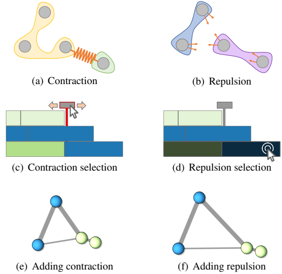
Fig. 6. Illustration of forces applied to the graph in Fig. 5(a). (a, c, and e): A contracting force applied to the layout. (b, d, and f): A repulsive force is then added to the layout from (e).
