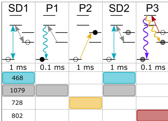
FIG. 2. The pulse sequence for the 2S_{1/2} \rightarrow 2D_{5/2} E2 transition measurement. Squiggly lines depict E1 allowed decays, straight lines show optical pumping transitions, and double-arrows indicate optical cycling transitions.
