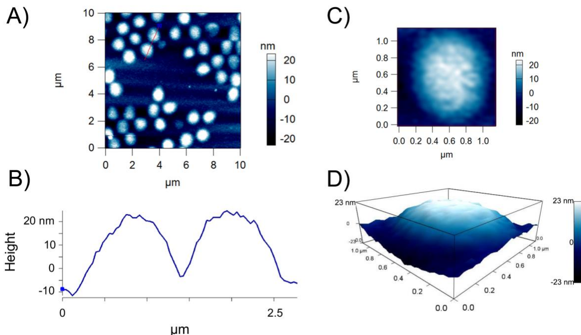
Figure 2: AFM characterization of ULC microgels deposited on a glass coverslip demonstrate ULC microgels are highly deformable. A) ULC microgels synthesized using 90% NIPAm and 10% AAc were deposited on a glass coverslip and imaged via AFM dry imaging. On glass surfaces, microgels were found to deform to have diameters on the order of 1 micron and B) to flatten to low heights of 26.5 \pm 21.7 nm. C) A representative single ULC microgel deposited on a glass coverslip. D) 3D map of the single ULC particle shown in part C. n = 30 particles analyzed.
