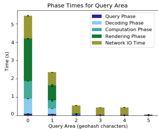
Figure 5: A comparison of data query times, separated by query phase, over different query areas. Network and query phase time are relatively constant, while the decoding, computation, and rendering phases dominate query time for large areas.
