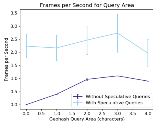
Figure 8: The number of frames in an animation that Aperture can display each second depending on the query area. Speculative queries have a major impact when the query area is relatively large, more than doubling the animation speed. Each frame consists of 3gb of unsketched data.
