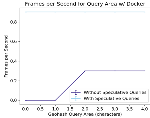
Figure 12: The number of frames in an animation that Aperture can display each second when run in a Docker container in a Kubernetes cluster. Animations load at 40% the speed they do without Docker.
