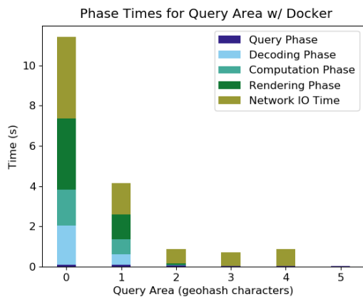
Figure 11: Aperture’s phase times when run from a Docker container in a Kubernetes cluster. The time for each phase is approximately doubled, with the exception of the query phase.
