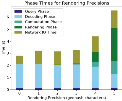
Figure 6: A comparison of data query times, separated by query phase, for different rendering precisions. At low values the precision is largely irrelevant, but it significantly increases the rendering and computation phase times at high values.
