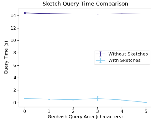
Figure 2: A comparison of the time Aperture takes to complete a query with and without Synopsis. Performing queries on sketches is more than 14 times faster than queries on un-sketched data.
