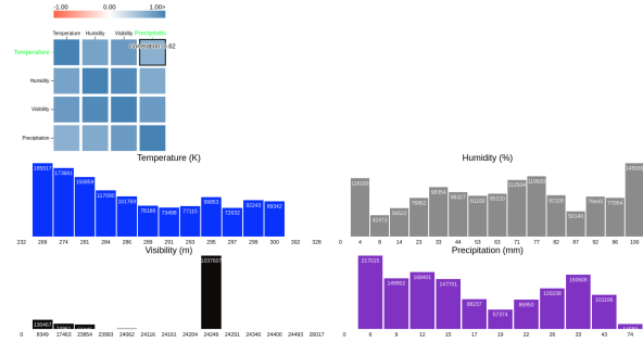
Figure 4: Aperture’s statistical views. The matrix shows the correlation score between every pair of features. The bar charts show the distribution of measurements for each feature.
