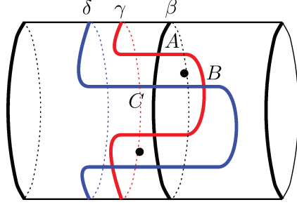
FIGURE 3. If \delta is obtained from \beta by a Hamiltonian isotopy supported away from the marked points, the domain of the distinguished triangle class in (\Sigma, \beta, \gamma, \delta, \mathbf{z}) connecting \Theta_{\beta\gamma} , \Theta_{\gamma\delta} and \Theta_{\beta\delta} will contain one of the marked points corresponding to the strands connected by \mathbb{I} . The intersection of the domain of the triangle with the surface is the small triangle connecting A , B and C .
