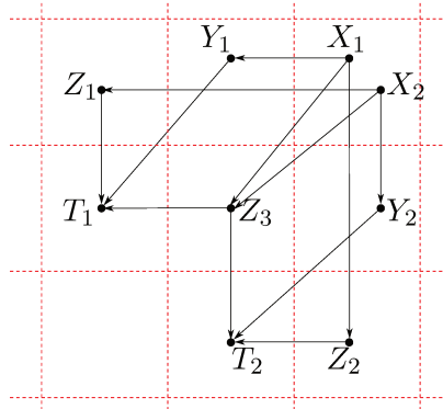
FIGURE 8. The chain complex associated with the knot T_{2,3;2,-1} .
