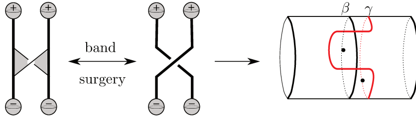
FIGURE 2. The right picture shows the two special \beta and \gamma curves corresponding to the band surgery on the Heegaard diagram subordinate to the band.
