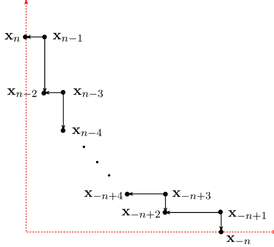
FIGURE 5. Each horizontal arrow from \mathbf{x}_i to \mathbf{x}_{i+1} has length a_{i+1} - a_i , while each vertical arrow from \mathbf{x}_i to \mathbf{x}_{i-1} has length a_i - a_{i-1} .
