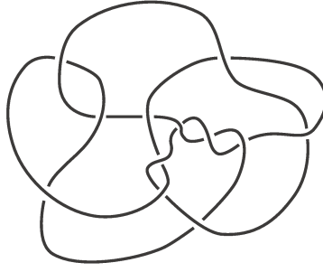
FIGURE 6. The knot 12n_{404}
