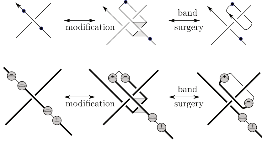
FIGURE 1. We may change a crossing in the expense of adding a meridian. The meridian can be positively or negatively oriented depending on whether the initial crossing is positive or negative, respectively.
