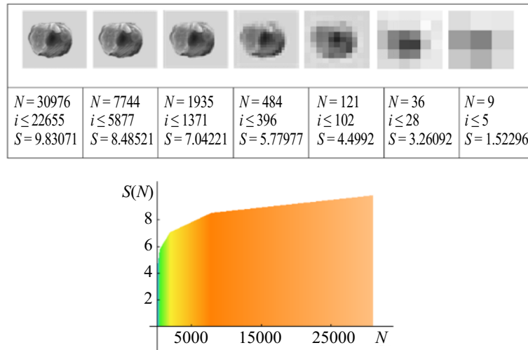
Figure 4. Shannon entropies from the table
