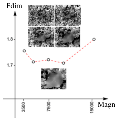
Figure 3. The diagram of fractal dimension vs. magnification shows variations
