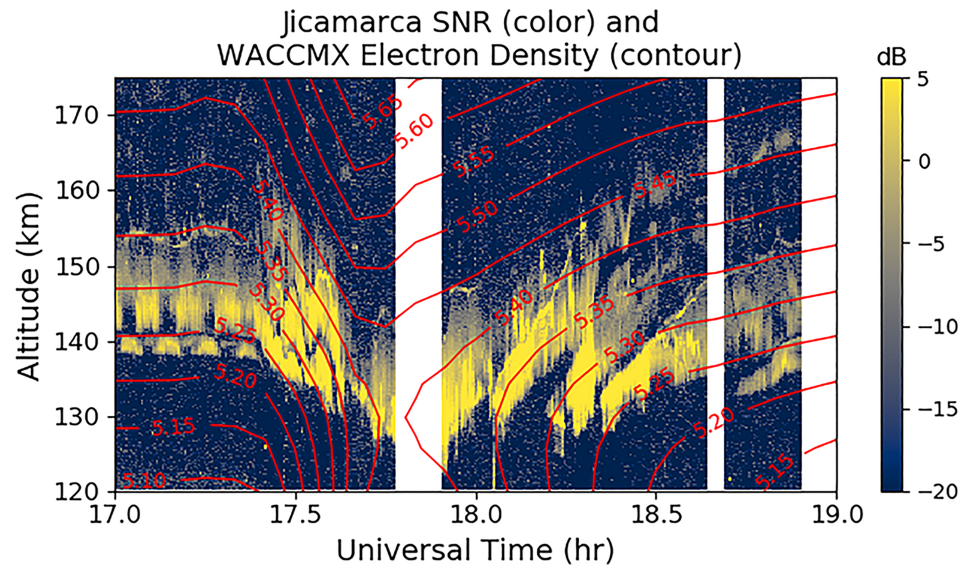
Figure 2. Observed signal-to-noise ratio (SNR; colors) and Whole Atmosphere Community Climate Model with thermosphere-ionosphere eXtension (WACCM-X) electron densities in units of \log_{10} \text{ cm}^{-3} (contours) during the 7 September 2005 solar flare.
