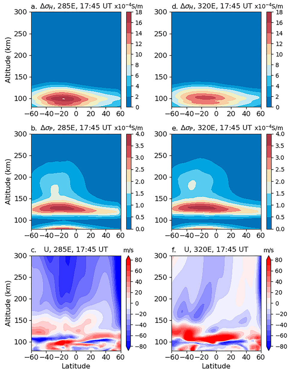
Figure 4. Changes in (a) Hall and (b) Pedersen conductivity at 285° E geographic longitude and 17:45 UT. (c) Zonal wind at 285° geographic longitude and 17:45 UT. (d–f) Same as (a)–(c) except for at 320° E geographic longitude.
