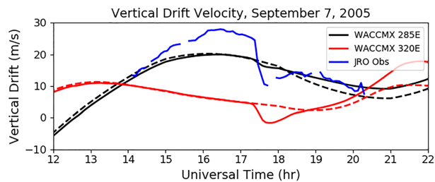
Figure 3. Equatorial vertical drift velocity on 7 September 2005 from Jicamarca 150-km echoes (blue) and Whole Atmosphere Community Climate Model with thermosphere-ionosphere eXtension (WACCM-X) simulations at 285° E (black) and 320° E (red) geographic longitude. Dashed lines indicate WACCM-X results without inclusion of the solar flare. JRO = Jicamarca Radio Observatory.
