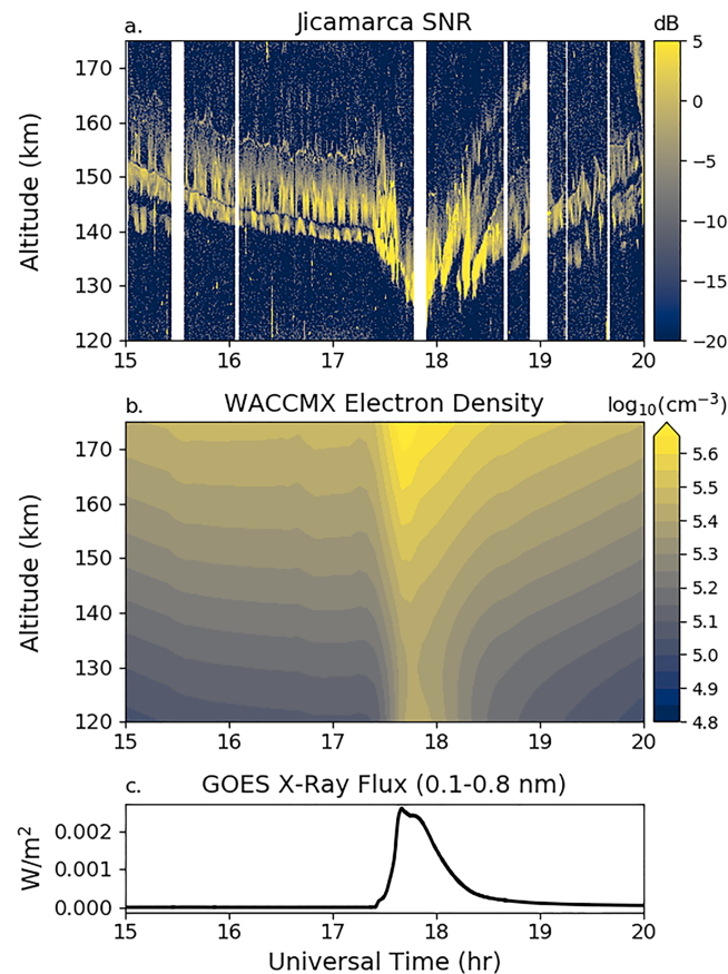
Figure 1. (a) Jicamarca Radio Observatory observed signal-to-noise ratio (SNR) during the 7 September 2005 solar flare. White areas indicate time periods without observations. (b) Electron densities simulated by Whole Atmosphere Community Climate Model with thermosphere-ionosphere eXtension (WACCM-X) at the location of Jicamarca, Peru. (c) Observed Geostationary Operational Environmental Satellite (GOES) X-ray flux for 0.1–0.8 nm.
