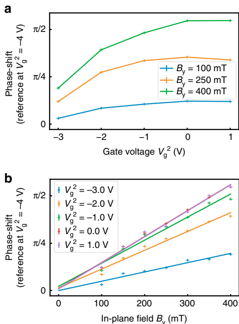
Fig. 4 Tuning anomalous phase shift using gate voltage and in-plane magnetic field. Evolution of the phase shift in JJ2 as a function of the gate voltage ( a ) and of the applied in-plane field along y ( b ). The phase shift \Delta\phi_0 is measured between the oscillations at a given value of V_g^2 and the ones at -4 V used as reference. In b the solid lines corresponds to linear fits to the measured phase shifts.
