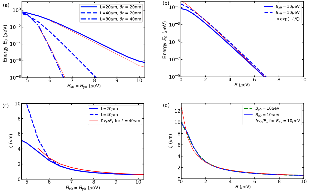
FIG. 5. (a) Numerically obtained value of the lowest positive energy E_0 as a function of the magnetic field amplitude B_{x0} = B_{y0} in wires of length L = 20 \mu\text{m} (solid line) and L = 40 \mu\text{m} (dashed line) obtained using \delta r = 20 \text{ nm} and L = 80 \mu\text{m} obtained using \delta r = 40 \text{ nm} . The onset of exponential decrease of E_0 with increasing B_{x0} = B_{y0} above \Delta indicates the transition to the topologically nontrivial superconducting phase, with the stronger dependence in longer wires arising because the overlap between MBS decreases exponentially with wire length. Thin red lines show E \propto \exp(-L/\xi) , where \xi is given by Eq. (27). (b) Numerically obtained value of the lowest positive energy E_0 in wires of length L = 40 \mu\text{m} as a function of the magnetic field amplitude B_{y0} (solid line) or B_{x0} (dashed line) fixed with B_{x0} = 2\Delta or B_{y0} = 2\Delta , respectively. The similarity of the behavior to that seen in (a) demonstrates the robustness of the topologically nontrivial phase to ellipticity in the helical magnetic field. Energy E_0 decreases exponentially as L/\xi is increased, as demonstrated by a thin red line for \propto \exp(-L/\xi) , where \xi is computed from Eq. (27) using E_1(B_{y0}) at B_{x0} = 2\Delta , see red solid line in Fig. 4(c). (c) Numerically obtained localization length of the lowest-energy state \zeta , obtained using Eq. (28) versus the strength of the magnetic field for a perfect helix, B_{x0} = B_{y0} , in wires of length L = 20 (solid line), 40 \mu\text{m} (dashed line). Also shown as the thin red line is the localization length \xi , Eq. (27), obtained using values of E_1 for a wire of length L = 40 \mu\text{m} , see red solid line in Fig. 4(a). (d) Numerically obtained localization lengths of the lowest-energy state, obtained using Eq. (28) versus the magnitude of B_{x0} (dashed line) or B_{y0} (solid line) with B_{y0} = 2\Delta or B_{x0} = 2\Delta , respectively, in wires of length L = 40 \mu\text{m} . Also shown as the thin red line is the localization length \xi obtained from Eq. (27) using E_1(B_{x0} = 2\Delta, B_{y0} = B) as a function of B , see solid red line in Fig. 4(b). The similarity to (c) demonstrates the robustness of the topological phase to ellipticity in the helical magnetic field. In all panels, superconducting gap parameter \Delta = 5 \mu\text{eV} and chemical potential \mu = \hbar^2 Q^2 / 8m = 49.6 \mu\text{eV} , which is matched to the middle of the magnetic superlattice gap.
